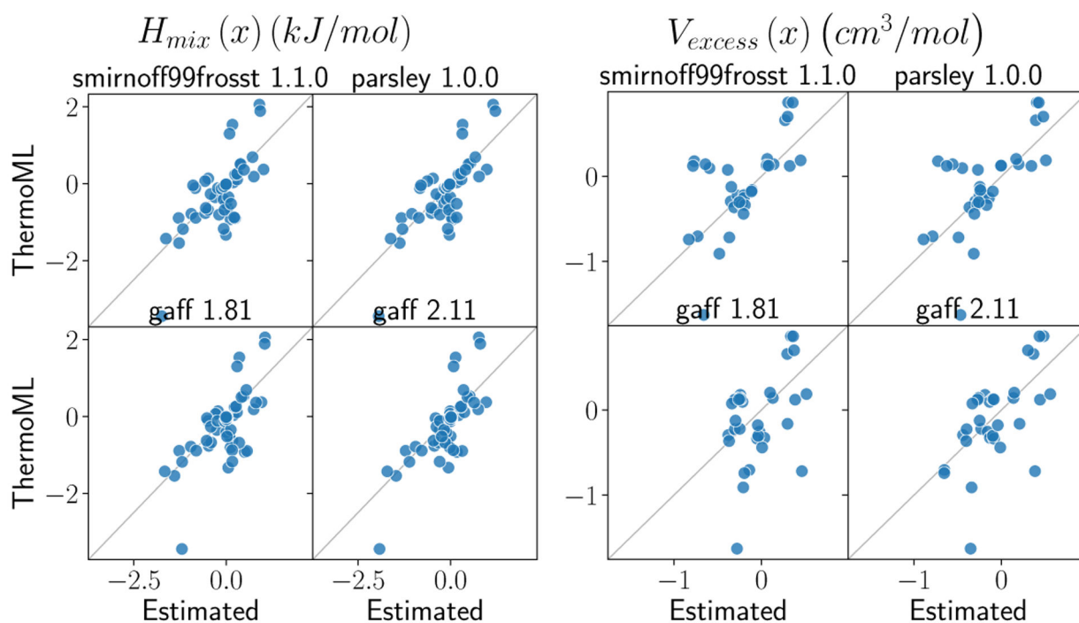
Figure 14. Results of binary mixture property benchmarks.
