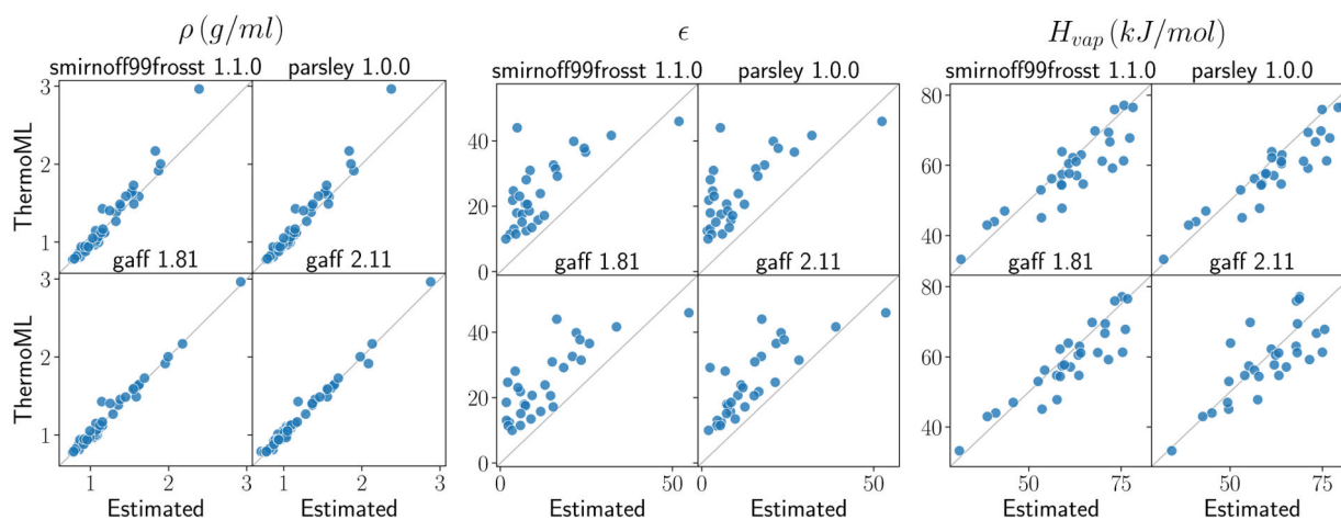
Figure 13. Results of pure property benchmarks.
