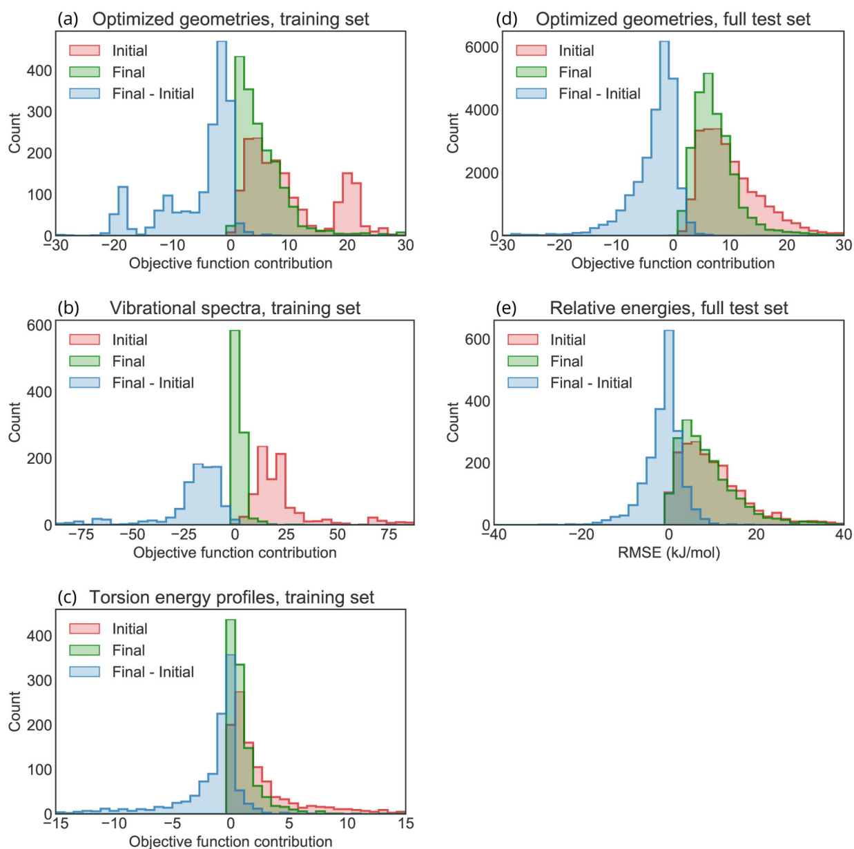
Figure 8. Improvement in components of the training set and test set objective functions with fitting.
