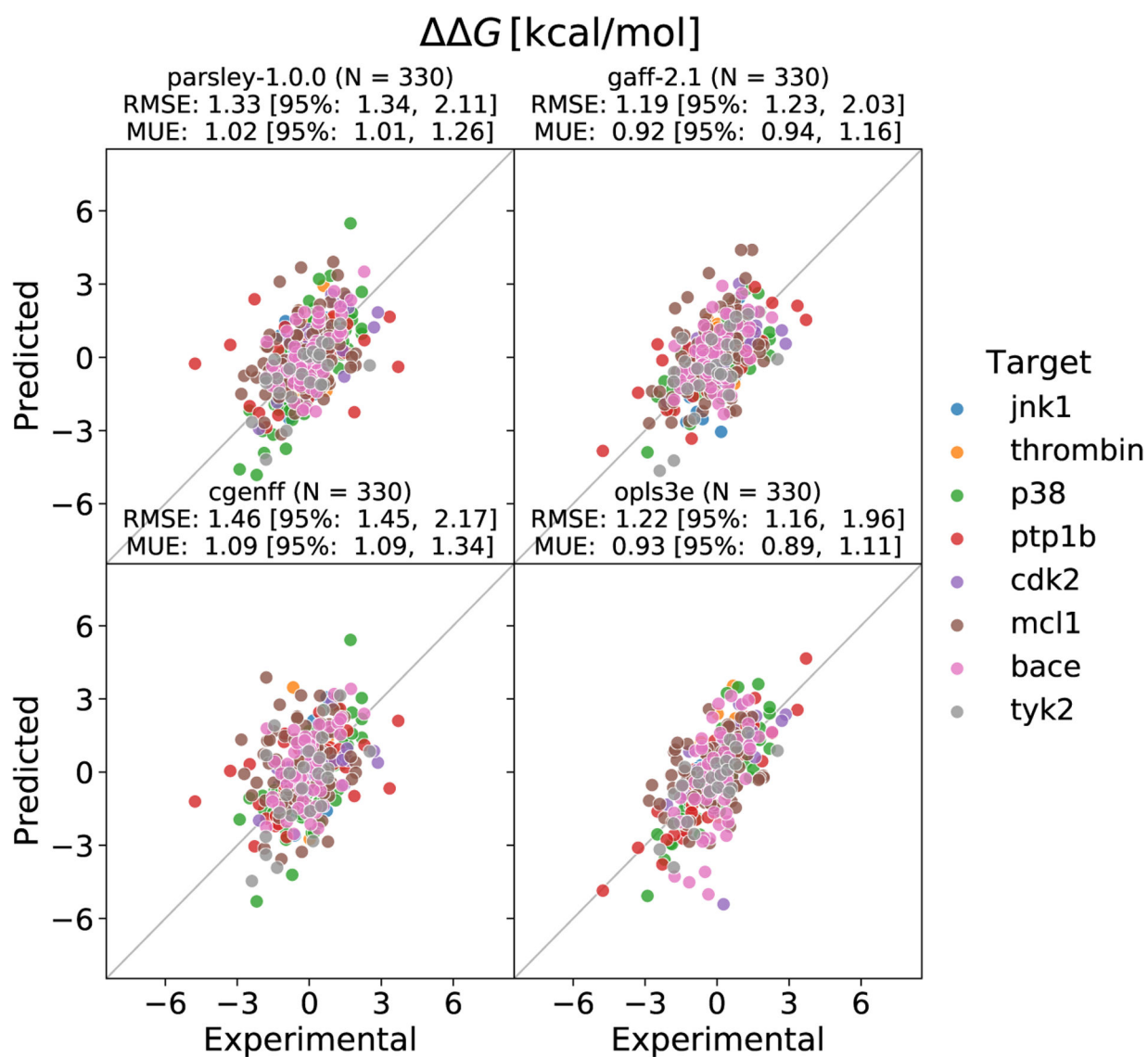
Figure 15. Results of protein-ligand binding free energy benchmarks.
