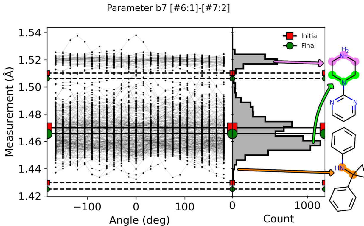
Figure 10. Dependence of bond lengths of a given force field type upon the chemical and conformational environment.
