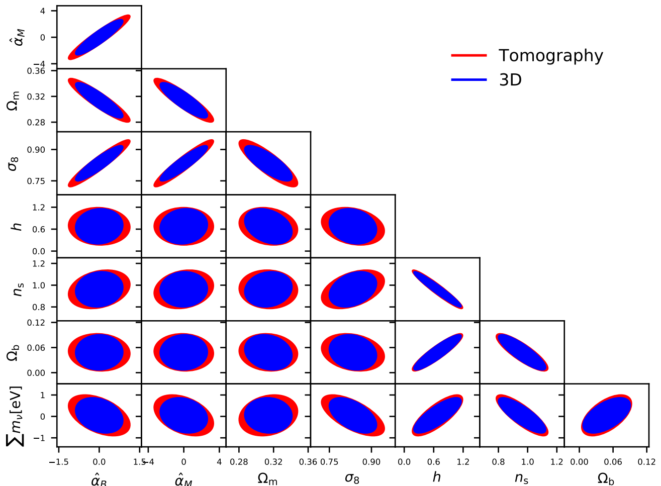
Figure 6. 1\text{-}\sigma forecast contours for a Euclid-like survey, showing a comparison between a fully 3D (blue) and a tomographic cosmic shear analysis (red). The fiducial values can be found in Table 2, while \hat{\alpha}_K = 0.01 and the survey specifications are given in Table 1. We used the linear matter power spectrum for both.
