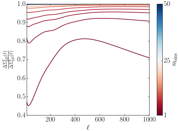
Figure 2. Differential signal-to-noise ratio of a tomographic analysis relative to a 3D analysis. The number of tomographic bins is shown in the colour bar.
