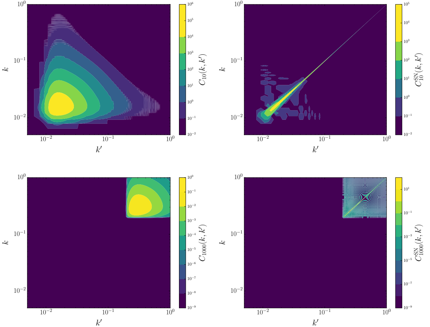
Figure 1. Signal (left, labelled C_\ell ) and noise (right, labelled C_\ell^{\text{SN}} , where the subscript stands for shot noise) parts of the covariance matrix (Eqs. 12 and 17, respectively) for the minimum and maximum \ell -mode considered in the analysis, \ell = 10 (upper panels) and \ell = 1000 (bottom panels), respectively. Note the different ranges of the colour bars, in logarithmic scale. See also Fig. 4 for a comparison between the diagonal elements of the matrices, highlighting how different multipoles have contributions with different orders of magnitude and how the signal and noise part become dominant for low and high \ell values, respectively.
