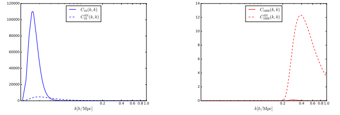
Figure 4. Comparison between the diagonal elements of the signal (solid line, as given by eq.12 and labelled C_\ell ) and noise (dashed line, as given by eq.17 and labelled C_\ell^{\text{SN}} , where the subscript stands for shot noise) contributions to the covariance matrices of the shear modes, for the minimum and maximum angular multipole considered in this analysis, i.e. \ell = 10 (blue) and \ell = 1000 (red), respectively. Note the different orders of magnitude for the different multipoles, and how the signal prevails on the noise for low multipoles, while the noise dominates for higher \ell values. Note also the log-scale on the x-axis, to help identify the different k -regions where most of the contributions come from, for different multipoles.
