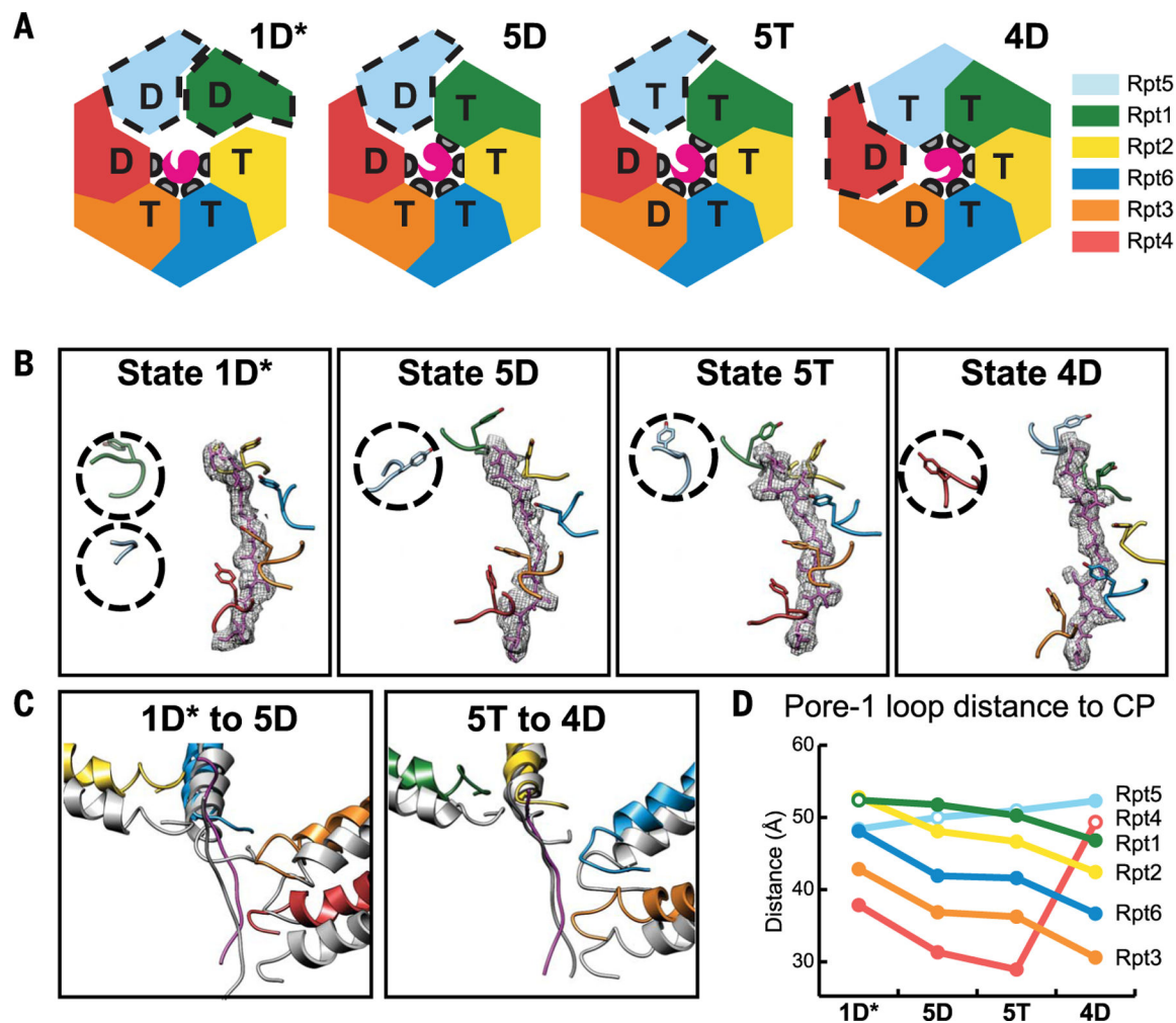
Fig. 3. Pore-1 loop tyrosines define three distinct spiral-staircase conformations of the AAA+ motor.
