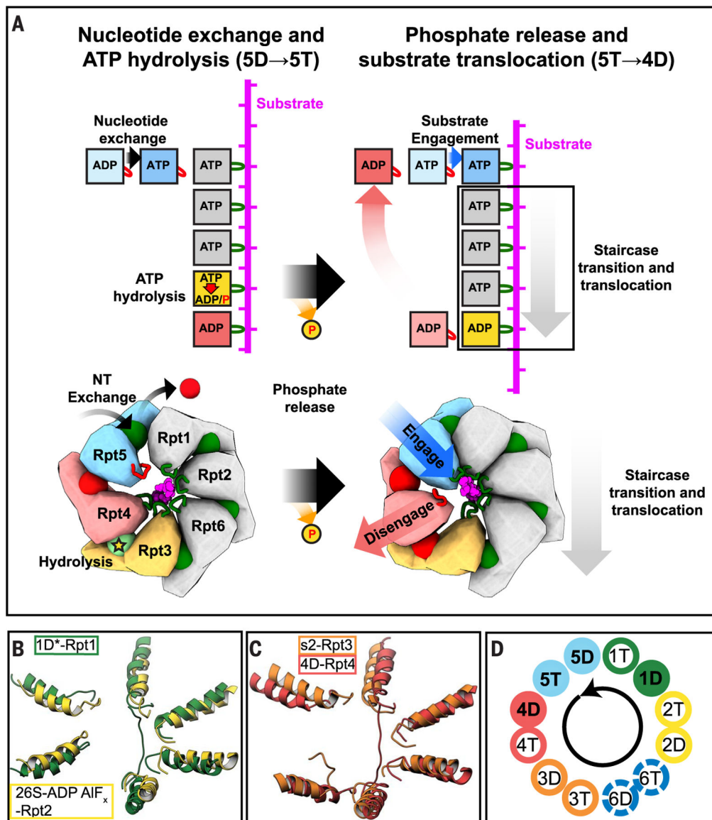
Fig. 4. Coordinated ATP-hydrolysis and substrate-translocation cycles of the proteasome. (A) Model for the coordination of ATP-hydrolysis steps and their coupling to substrate translocation. Nucleotide exchange and ATP hydrolysis occur simultaneously in the substrate-disengaged (blue) and penultimate subunit (orange) of the staircase, respectively, with no major conformational changes of the motor. Subsequent phosphate release from the penultimate subunit leads to the displacement of the bottom subunit (red), substrate-engagement by the top subunit (blue), and downward movement of a four-subunit rigid body (boxed) to translocate substrate. (B) Spiral staircases of 1D* (dark green) and the 26S-ADP-AIF x [yellow; PDB:5wvk (35)], rotated to overlay the disengaged subunits (1D*-Rpt1 and 26S-ADP-AIF x -Rpt2) and aligned by the pore-1 loop helices. (C) Spiral staircases of the s2 state [orange; PDB: (33)] and the 4D state, rotated to overlay the disengaged subunits (s2-Rpt3 and 4D-Rpt4) and aligned by the pore-1 loop helices. (D) Schematic of the possible progression of proteasome states, colored by the disengaged subunit, with our observed
