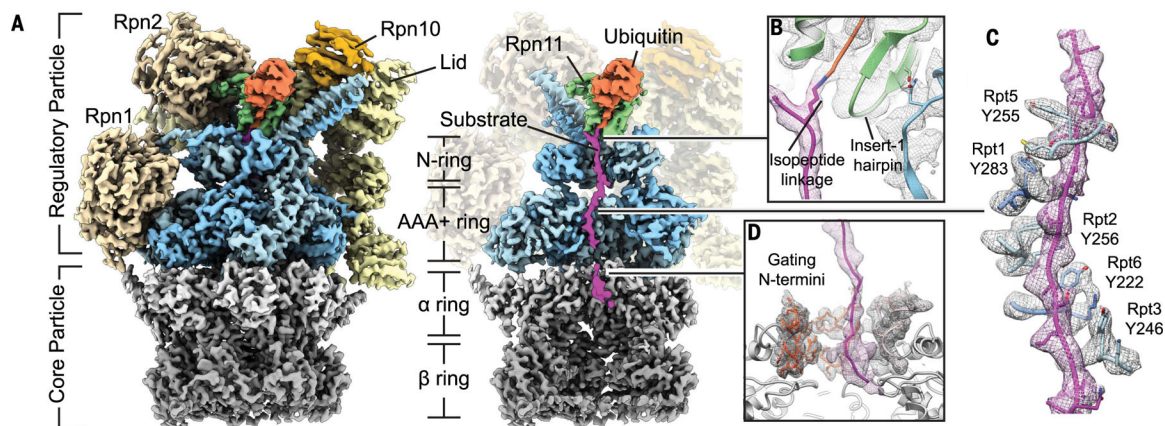
Fig. 1. High-resolution structure of the substrate-engaged 26S proteasome.
