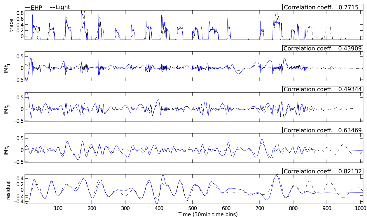
Figure 6.12: Decomposition of the EHP and light trace using bivariate EMD. IMFs correlation coefficients highlight the intrinsic relationship of the two traces.
