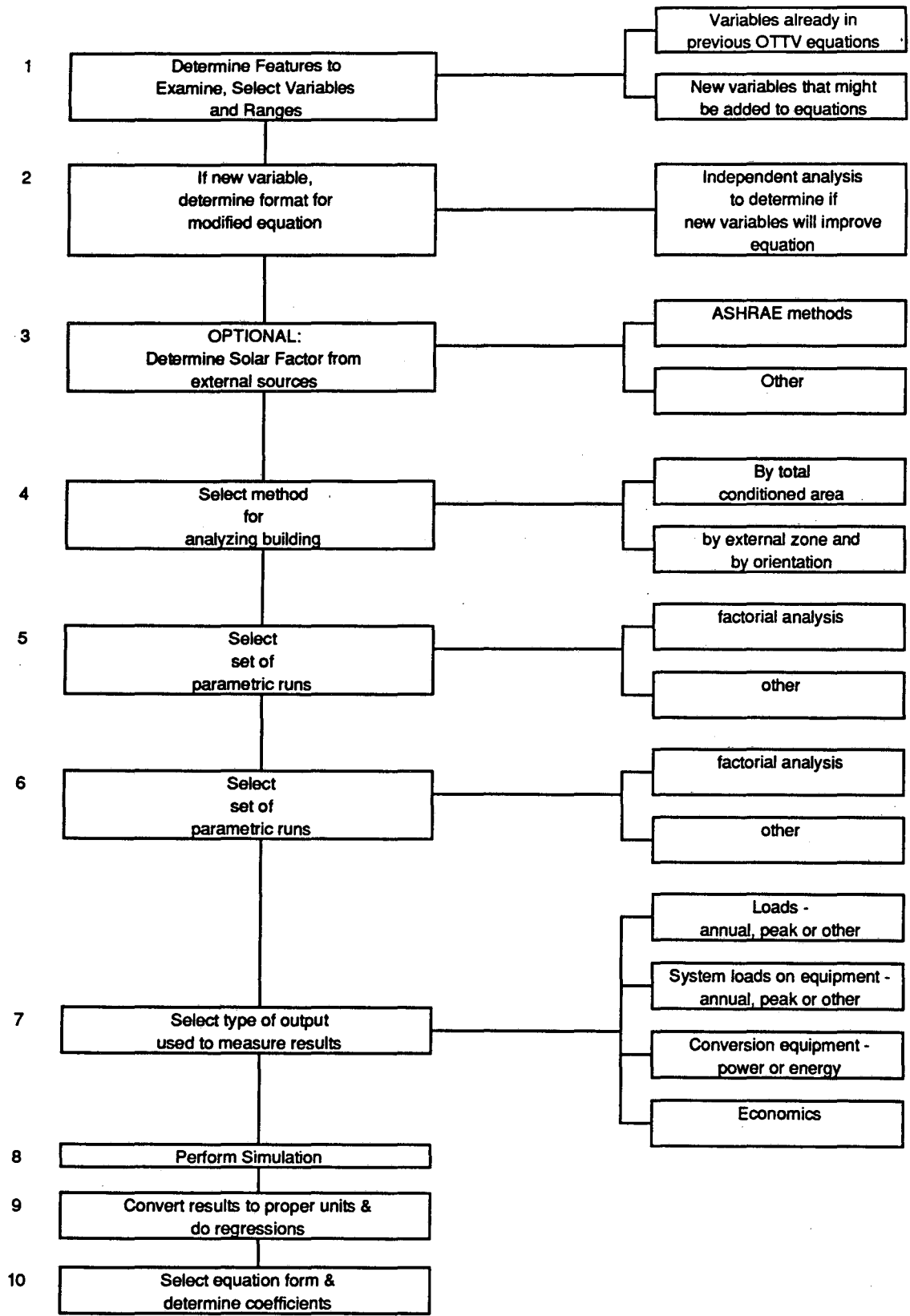
FIGURE 8-1. OTTV Analysis Procedure (for a single climate location)
