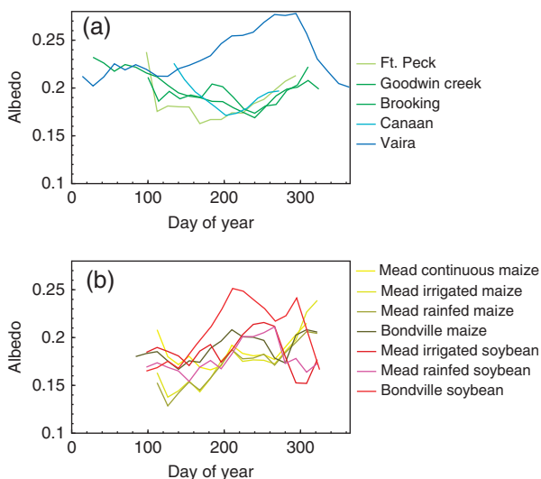
Fig. 3 Snow-free seasonal albedo integrated over 2-week periods for grasslands (a) and crops (b). Where multiple years of albedo data are available (e.g. Ft. Peck, Goodwin Creek), data from the year with the median albedo value for the biweekly period nearest day 200 are shown.
