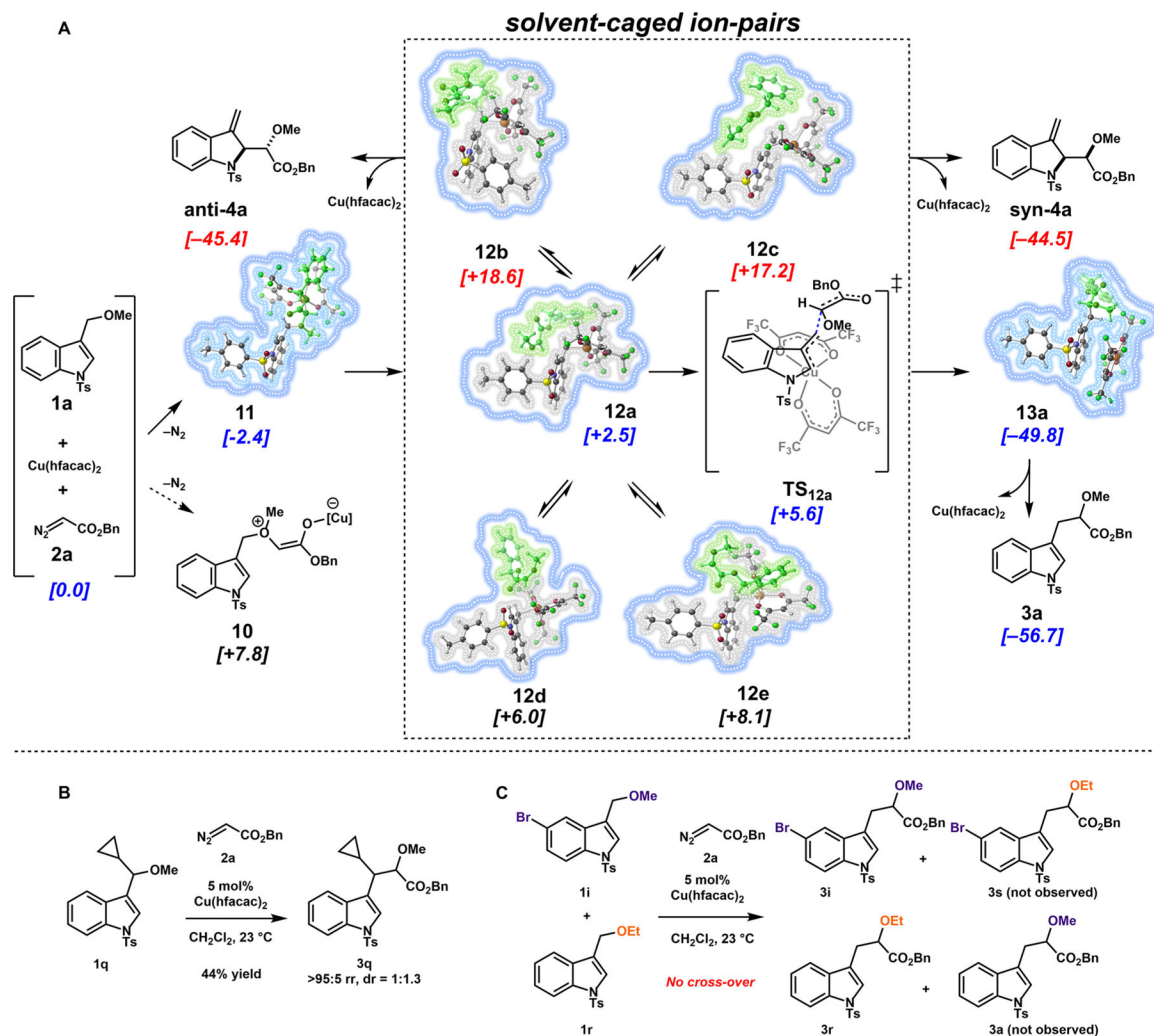
Figure 2. (A) Computed (PWPB95-D3(BJ)/def2-QZVPP//IEFPCM( \text{CH}_2\text{Cl}_2 )-B3LYP/6-31G(d),SDD) relative free energies (kcal/mol, italics) for minima and TSSs involved in the Cu-promoted reaction of 1a and 2a . A selection of ion-pairs 12a-12e were generated by scanning the bonds that form en route to the products. The energies for ion-pairs 12a-12e are based on optimized complexes. Geometries of ion-pairs 12a-12e , their preceding zwitterion 11 , and the recombination product 13a shown in ball-and-stick images are included to facilitate comparison of overall shapes. For clarity in visual comparison, the enolate part of the ion-pair is highlighted in green and the indolyl part (highlighted in gray) is positioned the same way for each structure above. The solvent cage (not modeled explicitly) is depicted in blue with dotted lines. (B) Reaction conditions for radical probe experiment: indole 1q (0.16 mmol), benzyl diazoester 2a (1.2 equiv, added using syringe pump as 0.2 M solution in \text{CH}_2\text{Cl}_2 at a rate of 2 mL/h), \text{Cu}(\text{hfacac})_2 (5 mol %), \text{CH}_2\text{Cl}_2 , 23 °C. (C) Reaction conditions for crossover experiment: indole 1i (0.08 mmol, 0.5 equiv), indole 1r (0.08 mmol, 0.5 equiv) benzyl diazoester 2a (1.2 equiv, added using syringe pump as 0.2 M solution in \text{CH}_2\text{Cl}_2 at a rate of 2 mL/h), \text{Cu}(\text{hfacac})_2 (5 mol %), \text{CH}_2\text{Cl}_2 , 23 °C.
