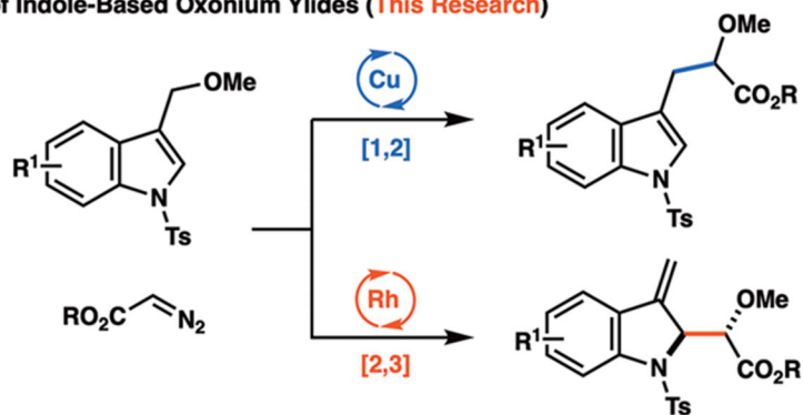
Scheme 1. Catalyst Control of Regioselectivity in Oxonium Ylide Rearrangements
