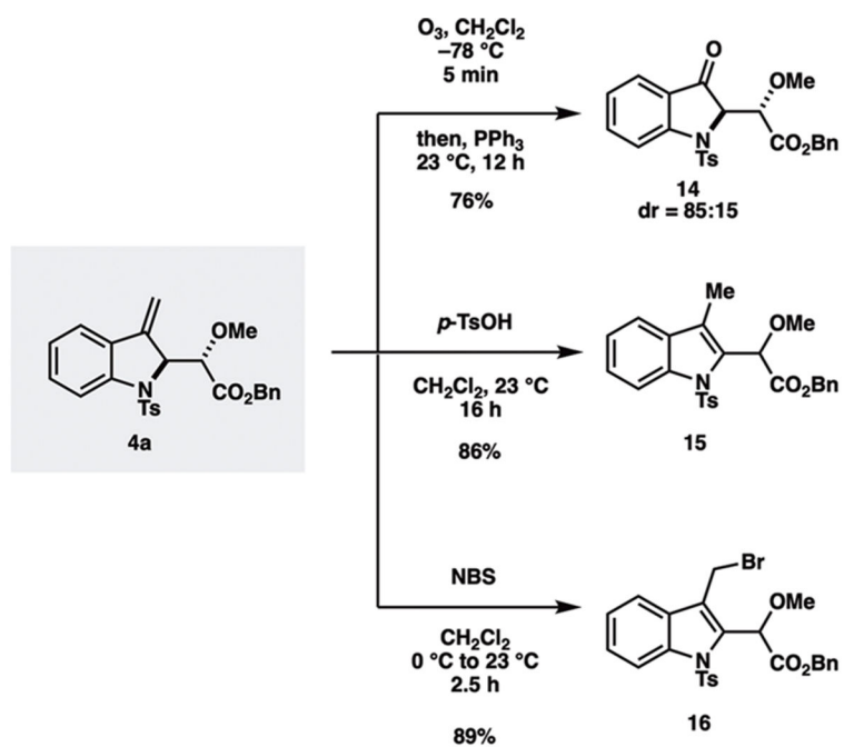
Scheme 2. Synthetic Derivatization of [2,3]-Rearrangement Product
