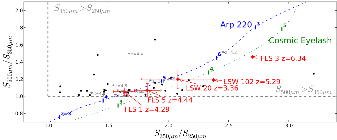
Figure 5. SPIRE color ratios for sources presented in this paper (black dots). The sources with redshifts are shown as red diamonds. For comparison, 500 \mu\text{m} -riser sources with redshifts selected via other methods (i.e., not on the basis of their SPIRE colors) are shown as gray stars (see §6). SED tracks based on Arp 220 and the Cosmic Eyelash (Swinbank et al. 2010) are shown for comparison. They gray dashed lines represent our selection in color space. Note that the uncertainties vary considerably, and are quite large for some of the sources. Example uncertainties are shown for FLS 1, 5, and LSW 20.
