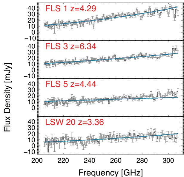
Figure 6. Z-Spec observations of our sources. All four have known redshifts from either CARMA or Keck as described in the text. Line searches in these data will be discussed in Riechers et al. 2013, in preparation.
