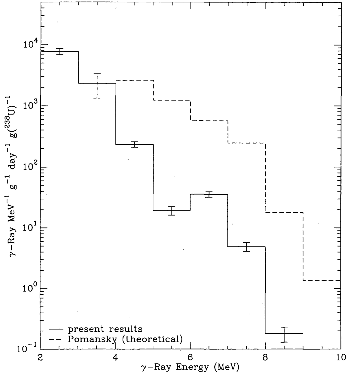
Fig. 6. The direct \alpha -induced \gamma -ray spectrum in granite. The yields are reported in terms of the mass fraction of {}^{238}\text{U} , with a concentration of {}^{232}\text{Th} five times that of {}^{238}\text{U} . The solid histogram shows the spectrum derived from experimental measurements. The broken-line histogram shows the theoretical calculations of Pomansky for granite with the same radioactive content.
