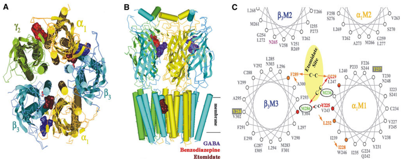
Fig. 1 Three-dimensional views of the \gamma -aminobutyric acid type A receptors (GABA A R) homology model from different perspectives (A,B) and helical wheel representation of the transmembrane regions at the etomidate binding domain at the \beta/\alpha interface (C). A) Three-dimensional view of the GABA A R homology model ( \beta_3 , cyan; \alpha_1 , yellow; \gamma_2 , green) from a perspective outside the membrane looking down the channel or B) from a perspective parallel to the membrane surface. Modified from Li et al. (2006) 29 in which our homology model is based roughly on the nicotinic acetylcholine receptor cryo-EM derived structure (PDB:2BG9), 47 modified by helical alignment data from Jansen & Akabas (2006). 51 Pockets in the vicinity of the etomidate (maroon), GABA (purple), and benzodiazepine (red) binding sites are shown as Connolly surfaces. C) Helical wheel
