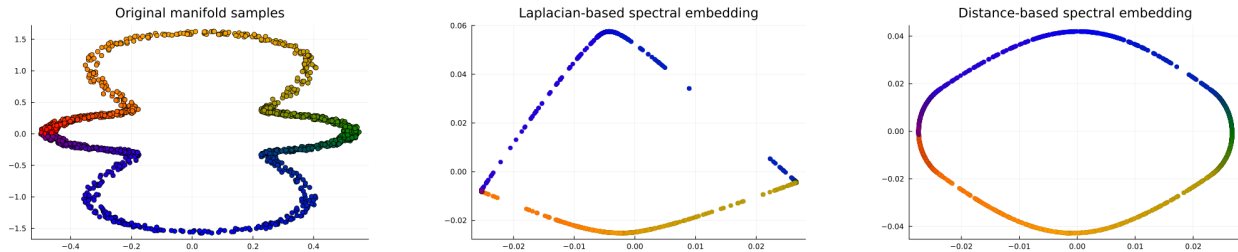
FIGURE 3.2. A demonstration of the similar basic capabilities of the Laplacian and discrete integral operator-based spectral embeddings. On the left is noisy samples of a manifold, and on the right, two-dimensional spectral embeddings utilizing appropriate eigenvectors of the Laplacian and discrete integral operator, respectively.
