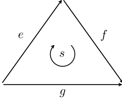
FIGURE 4.2. A naturally-oriented 2-simplex s , with naturally-oriented 1-faces e, f, g .
