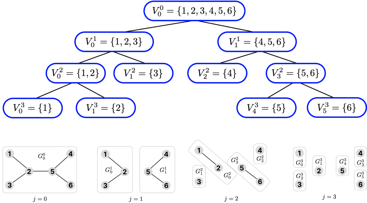
FIGURE 2.3. A hierarchical partition tree, for the 6 vertices of a simple example graph. In the tree above, the root is V_0^0 , containing all the vertices, and each next level of the tree contains subsets at common scale. The leaves of the tree are singleton subsets. In the graphs below, the regions G_k^j induced by the corresponding vertex subsets V_k^j are demonstrated.
