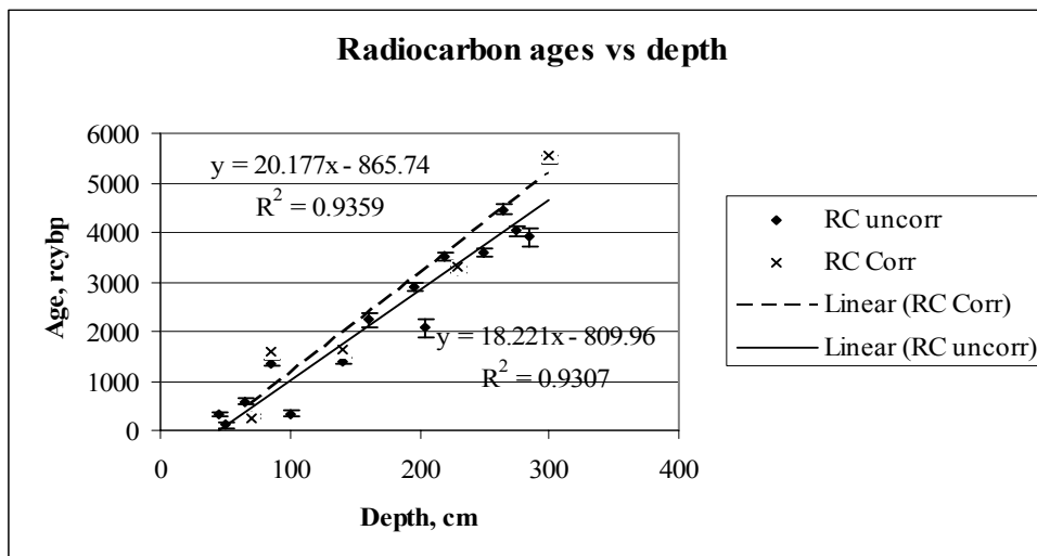
Figure 2. Rose Spring radiocarbon ages plotted against depth.
