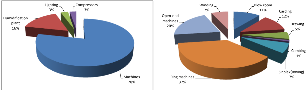
Figure 7. Breakdown of the Final Energy use in a Spinning Plant that has both Ring and Open-End Spinning Machines [120]
