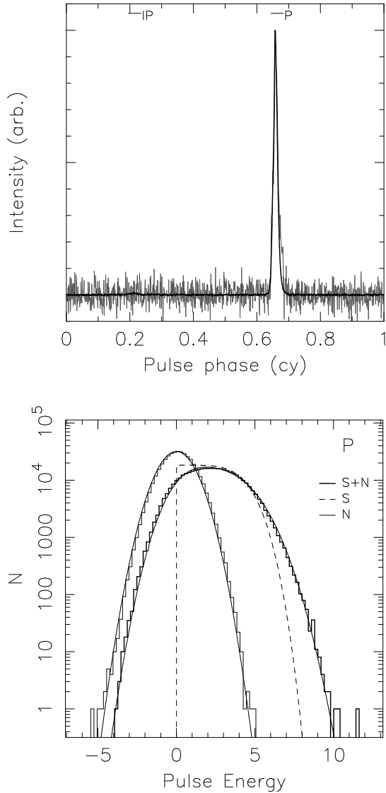
Figure 14. Upper panel: Pulse profiles for PSR J1909–3744. The thick line shows the average pulse profile formed from all of our single-pulse observations. The thinner grey line shows the average of the 100 brightest pulses. The profiles have been normalised to have the same peak flux density. Lower panel: Pulse-energy distribution in window P for PSR J1909–3744. The labels are the same as in Figure 2.
