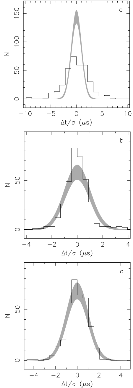
Figure 22. Histograms of normalised residuals for PSR J0437–4715. Panel a): No modification to TOA uncertainties Panel b): Adding in quadrature 100 ns to the TOA uncertainties. Panel c): Modifying TOA error using Equation (16). The grey shaded area represents the range in the histogram theoretically expected.
