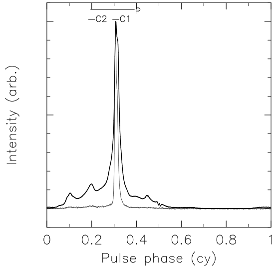
Figure 5. Pulse profiles for PSR J0437–4715. The thick line shows an average pulse profile for PSR J0437–4715 formed from all of our single-pulse observation. The thinner grey line shows the profile formed from 100 most energetic pulses. The profiles have been normalised to have the same peak flux density.
