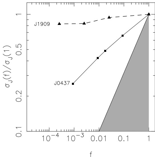
Figure 23. Fraction of pulses used versus normalised timing error for PSR J0437–4715 (labelled J0437) and PSR J1909–3744 (labelled J1909). The filled grey area identifies the region \sigma_J(1, f) < \sigma_J(1, 1)/\sqrt{f} , in which precision timing would benefit from using fewer pulses.
