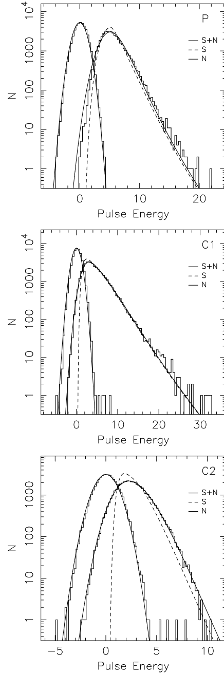
Figure 18. Pulse-energy histograms for PSR J2145–0750. In the uppermost panel, we show the pulse-energy distribution for the main pulse, identified as region P in the upper panel of Figure 17. In the centre and lowermost panels we show respectively the pulse-energy distribution in windows C1 and C2, also labelled in Figure 17, centred on components C1 and C2. See Figure 2 for a description of the plot.
