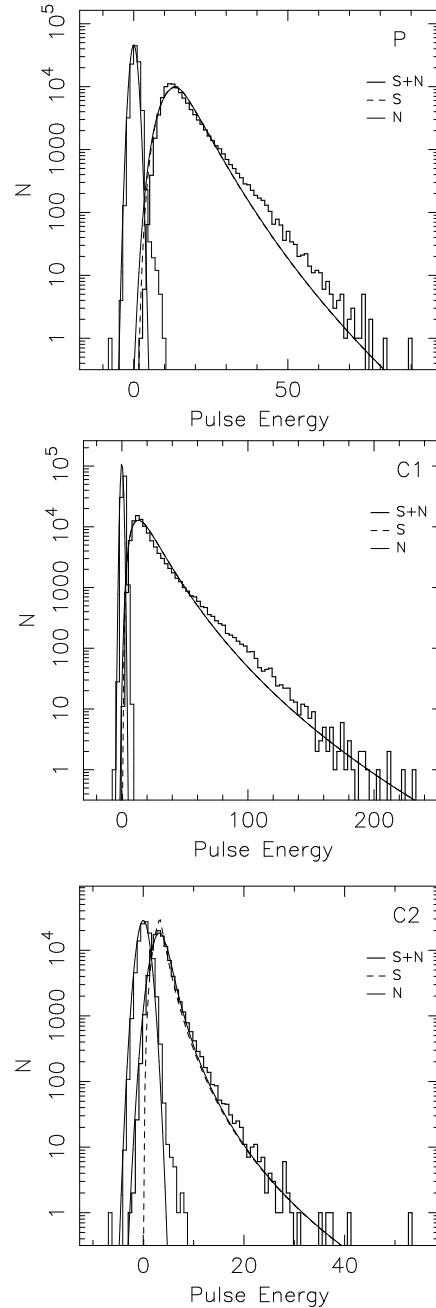
Figure 7. Pulse-energy histograms for PSR J0437–4715. The uppermost panel shows the histogram for a window containing the brightest part of the pulse profile (labelled P in the upper panel of Figure 5), the middle panel shows the distribution for a window centred on component C1, and the lowermost panel shows the distribution for a window centred on component C2. The labels are the same as in Figure 2.
