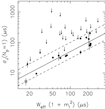
Figure 20. Correlation of pulse width W_{\text{eff}}(1 + m_I^2) and level of jitter noise \sigma_J(N_p = 1) . The downward pointing arrows show upper limits on the levels of jitter noise. The lines represent different models \sigma_J = \bar{f}_J W_{50} , where \bar{f}_J is the mean value for the relationship. The solid line is the best-fitting value \bar{f}_J = 0.5 \pm 0.1 , the lower and upper dashed lines show the trends \bar{f}_J = 0.3 and \bar{f}_J = 1.0 respectively. The open square show measurements of jitter noise for PSR J1939+2134 at 1400 MHz, while the filled circle shows excess noise at 730 MHz that we attribute to the effects of stochastic pulse broadening.
