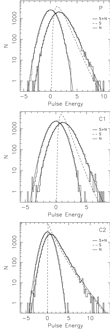
Figure 10. Pulse-energy distributions for PSR J1022+1001. In the uppermost panel, we show the energy distribution over the majority of the pulse (window P in Figure 9), in the middle panel we show the energy distribution for a window C1 centred on the leading component, and in lowermost panel we show the energy distribution in a window C2 centred on the trailing component. The labels are the same as in Figure 2.
