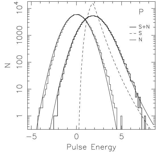
Figure 2. Pulse-energy histograms for PSR J1713+0747. The thick solid histogram shows the pulse-energy histogram in the on pulse window. The thick solid line (labelled S+N) is the best-fitting model to the distribution. The on pulse window is labelled P in Figure 1. The thin solid histogram and line (labelled N) show, respectively, the histogram for the off-pulse window and the predicted normal Gaussian distribution. The units of pulse energy have been scaled to the rms of the off-pulse window. The thin dashed line (labelled S) shows the intrinsic pulse-energy histogram, deconvolved using Equation (7).
