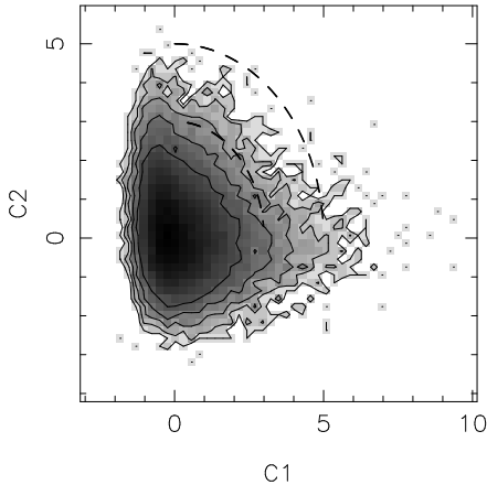
Figure 19. Correlations in energy of components C1 and C2 for PSR J2145–0750. The components have been normalised to have unit mean and variance. The dashed lines shows the (1-\sigma) and (2-\sigma) contour of equal probability if component energies are independent.
