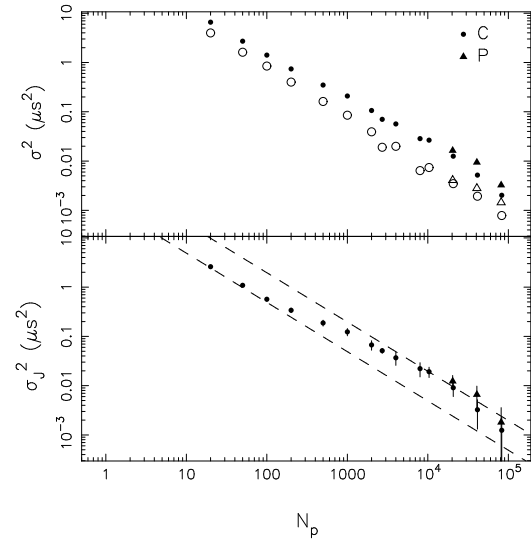
Figure 15. Estimates of levels of jitter noise for PSR J1909–3744. Upper panel: Variance of residual time series for observed datasets (filled symbols) and simulated datasets (open symbols). The symbols shapes represent different backends and are listed below. Lower panel: the difference between the observed and simulated variance. We attribute this difference to pulse-shape variations. The dashed lines show the levels of jitter noise predicted from observations of < 10^3 pulses (lower line) and > 10^4 pulses (upper line), both scaling \propto N_p^{-1/2} . Symbols: circles - CASPSR at 1400 MHz (labelled C); triangles - PDFB3 at 1400 MHz (labelled P).
