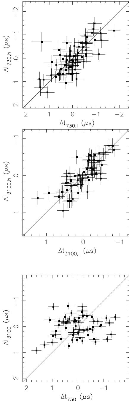
Figure 8. Correlation of residual TOAs for PSR J0437–4715. In the uppermost panel, we show the correlation between residuals formed from the lower half \Delta t_{730,l} and upper half \Delta t_{730,h} of the 730 MHz (50cm) band. In the middle panel, we show the correlation between residuals formed from the lower half \Delta t_{3100,l} and upper half \Delta t_{3100,h} of the 3100 MHz (10cm) band. In the bottom panel, we plot residuals formed at 730 MHz ( \Delta t_{730} ) and 3100 MHz ( \Delta t_{3100} ) observations. In all of the panels, the solid lines denote unit correlation.
