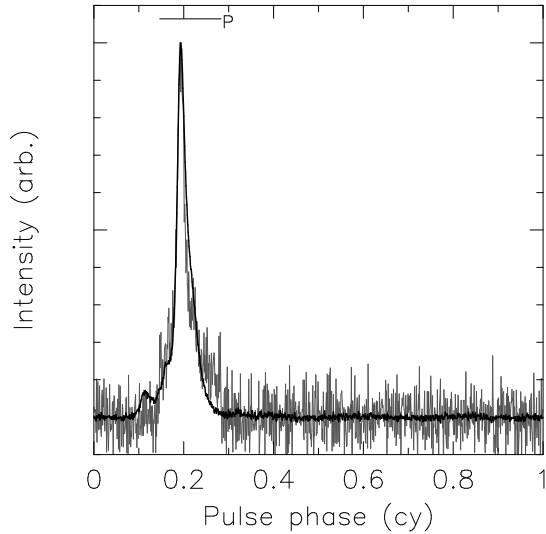
Figure 1. Pulse profiles for PSR J1713+0747. The thick line shows the average pulse profile for PSR J1713+0747, derived from averaging our single-pulse observations. The thinner grey line shows the pulse profile formed from 100 most energetic single pulses for PSR J1713+0747. The profiles have been normalised to have the same peak flux density. The horizontal line labelled P shows the pulse window used to measure pulse energy (see Figure 2).
