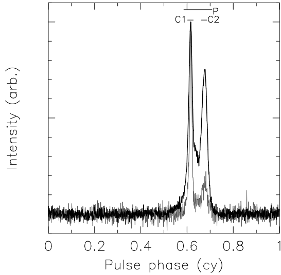
Figure 11. Pulse profiles for PSR J1603–7202. The thick line shows the average pulse profile formed from all of our single-pulse observations. The thinner grey line shows the average of the 100 brightest pulses. The profiles have been normalised to have the same peak flux density.
