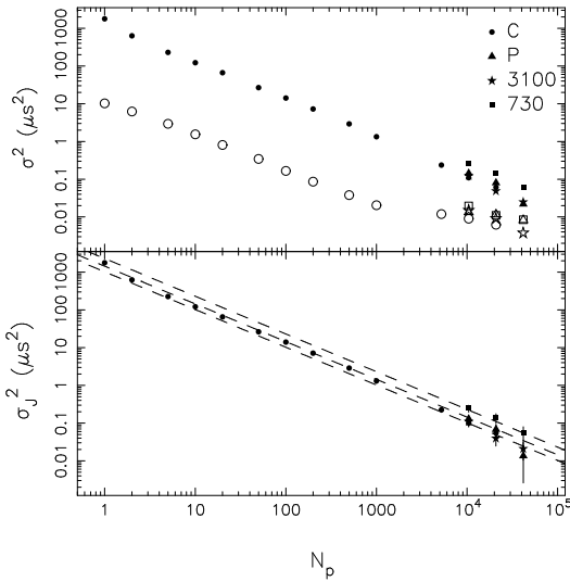
Figure 6. Estimates for levels of jitter noise in PSR J0437–4715. Upper panel: Variance of residual time series for observed datasets (filled symbols) and simulated datasets (open symbols) from observations with the Parkes Telescope. Lower panel: The quadrature difference between the observed and simulated datasets, \sigma_J(N_p) . Symbols: squares - 50cm/PDFB3 observations at 730 MHz (labelled 730); stars - 10cm/PDFB4 observations observing at 3100 MHz (labelled 3100); circles - Parkes/CASPSR observing at 1400 MHz (labelled C); triangles - Parkes/PDFB4 observing at 1400 MHz (labelled P). The top dashed line shows the fitted jitter model for the 50cm data. The middle dashed line shows the fitted jitter noise to the 20cm data. The bottom dashed line shows the fitted jitter model for the 10 cm observations
