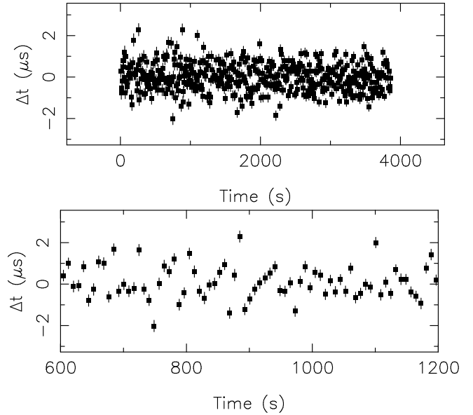
Figure 4. Top panel: Residual arrival times for 3840 s observation of PSR J1713+0747, derived from CASPSR observations with 8 s subintegrations. Bottom panel: Sub-interval highlighting drift in arrival times over \sim 48 s at a time of 900 s.
