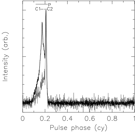
Figure 9. Pulse profiles for PSR J1022+1001. The thick line shows the average pulse profile formed from all of our single-pulse observations. The thinner grey line shows the average of the 100 brightest pulses. The profiles have been normalised to have the same peak flux density.
