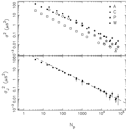
Figure 3. Estimates of jitter noise in PSR J1713+0747. Upper panel: Variance of residual time series versus number of pulses averaged N_p for observations (filled symbols) and simulated datasets (open symbols) from observations with the Parkes Telescope and the Arecibo Telescope. Because the data were obtained with telescopes with different sensitivities, the observed and simulated time series contain different levels of white noise. Lower panel: \sigma_J(N_p) , the quadrature difference between the observed and simulated datasets. The dashed line is the best fitting model for the jitter noise scaling \propto N_p^{-1/2} . Symbols: squares - Arecibo/WAPP Observations (labelled W, autocorrelation spectrometer) observing at 1600 MHz; stars - Arecibo/ASP (labelled A, a coherent dedispersion machine, using single channel of 4 MHz of bandwidth) observing at 1400 MHz; circles - Parkes/CASPSR observing at 1400 MHz (labelled C); triangles - Parkes/PDFB4 observing at 1400 MHz (labelled P)
