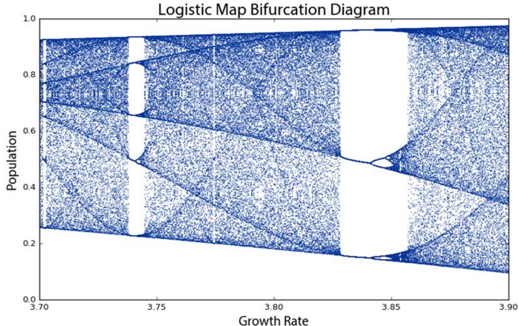
Figure 2.4. Bifurcation diagram of 100 generations of the logistic map for 1,000 growth rate parameter values between 3.7 and 3.9. The system moves from order to chaos and back again as the growth rate is adjusted.
