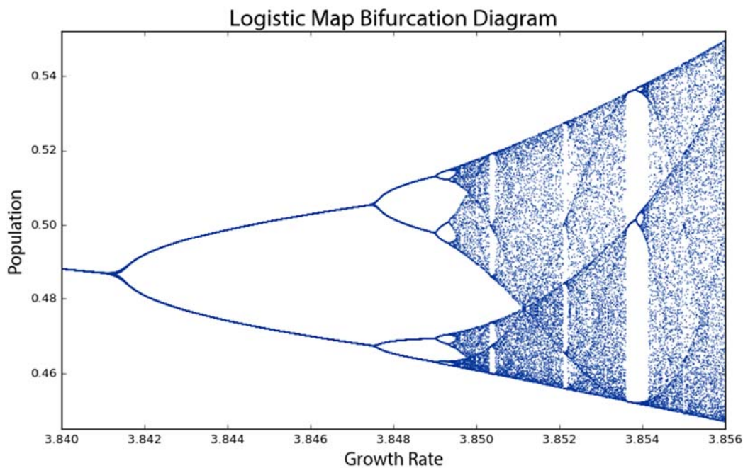
Figure 2.5. Bifurcation diagram of 100 generations of the logistic map for 1,000 growth rate parameter values between 3.84 and 3.856. This is the same structure that we saw earlier at the macro-level in Figure 2.3, because chaotic systems' strange attractors are fractal.
