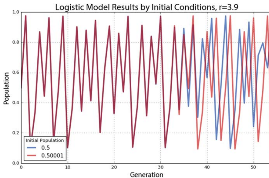
Figure 2.13. Plot of two time series with identical dynamics, one starting at an initial population value of 0.5 (blue) and the other starting at 0.50001 (red). At this growth rate parameter value of 3.9, the Lyapunov exponent is positive – thus the system is chaotic and we can see the nearby points diverge over time.
