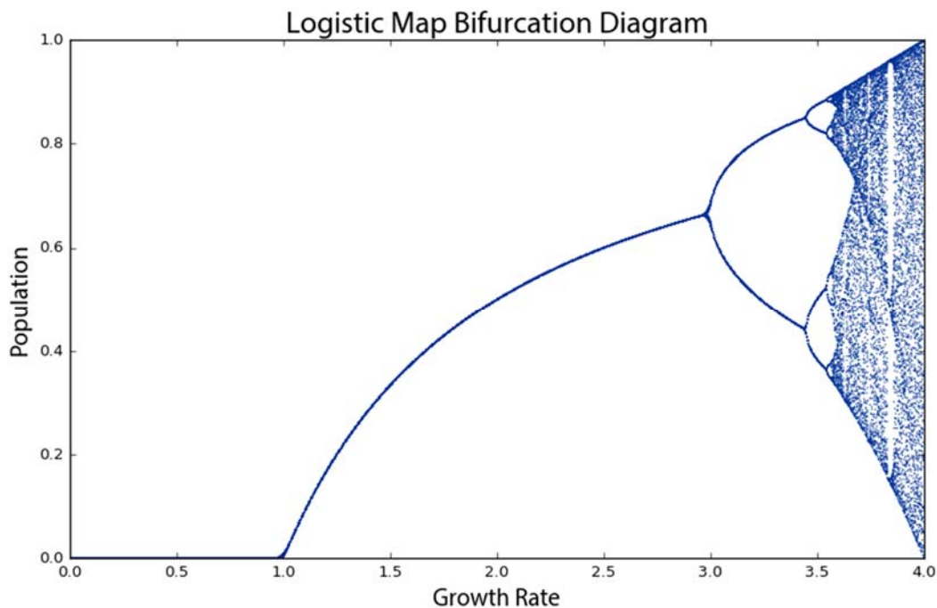
Figure 2.2. Bifurcation diagram of 100 generations of the logistic map for 1,000 growth rate parameter values between 0 and 4. The vertical slice above each growth rate depicts the system's attractor at that rate.
