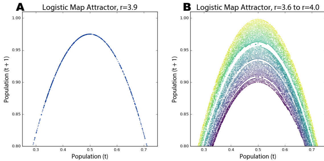
Figure 2.7. Cropped phase diagrams of the logistic map over 200 generations for (A) a growth rate parameter value of 3.9 and (B) 50 growth rate parameter values between 3.6 and 4 (the chaotic regime), each with its own colored line.
