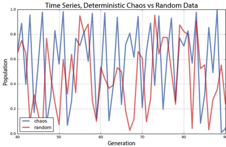
Figure 2.9. Plot of two time series, one deterministic/chaotic from the logistic map (blue), and one random (red).
