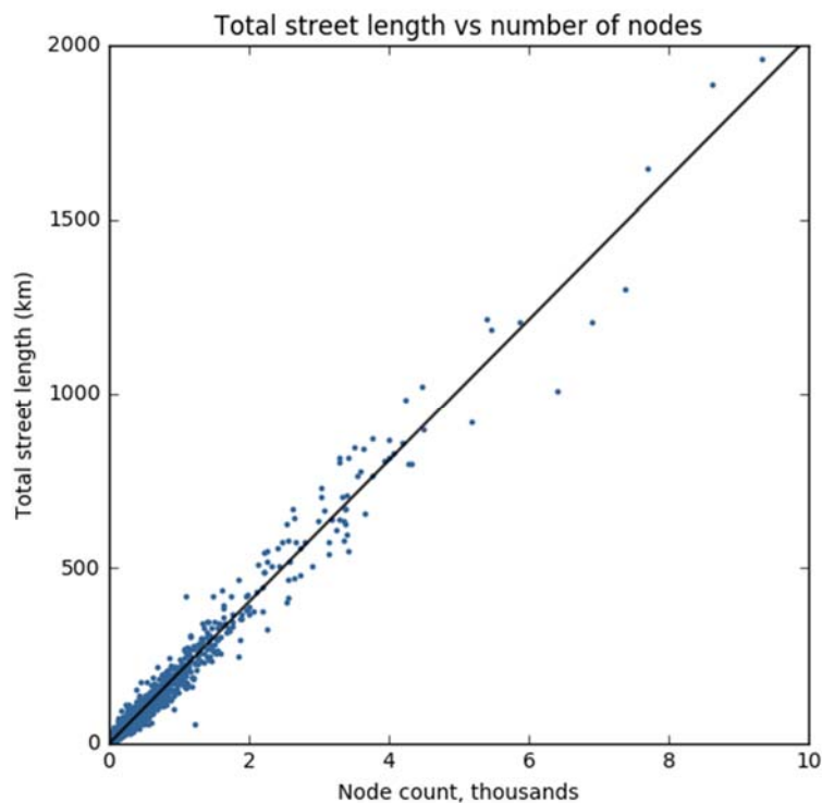
Figure 7.9. Relationship between total street length and number of nodes in neighborhood-scale street networks.
