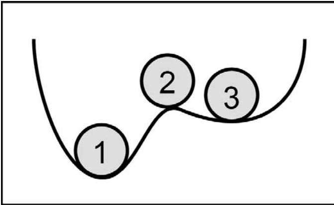
Figure 3.2. Three balls at rest on a slope, representing stable (ball 1), unstable (ball 2), and metastable (ball 3) states. Ball 1 will return to its current state after a large perturbation. Ball 2 will move away from its current state after even a slight perturbation. Ball 3 will remain in its current state after a small perturbation, but a large one can push it into a preferred stable state. Its semi-stable state is near a critical point of transition.
