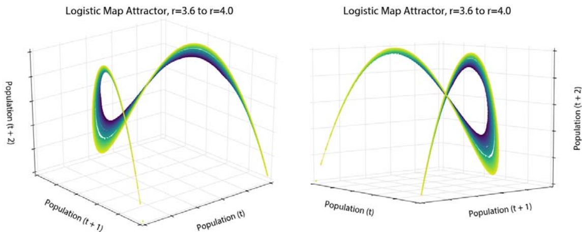
Figure 2.11. Two different viewing perspectives of a single three-dimensional phase diagram of the logistic map over 200 generations for 50 growth rate parameter values between 3.6 and 4, each with its own colored line.
