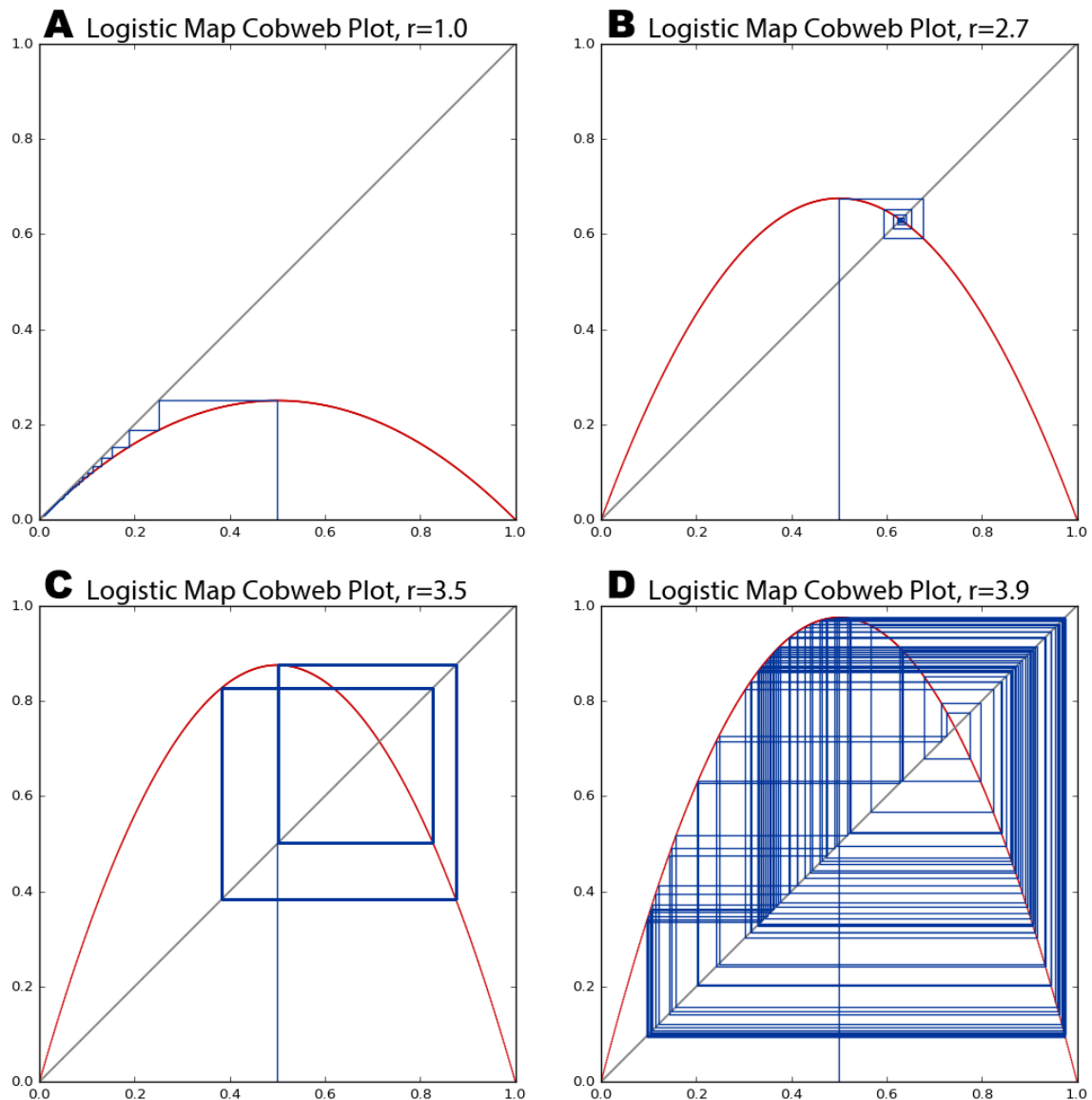
Figure 2.8. Cobweb plots of the logistic map for growth rate parameter values of (A) 1, (B) 2.7, (C) 3.5, (D) 3.9. The diagonal gray identity line represents y=x , the red curve represents the logistic map as y=f(x) for each of the four parameter values, and the blue line represents the system's trajectory over 100 generations.
