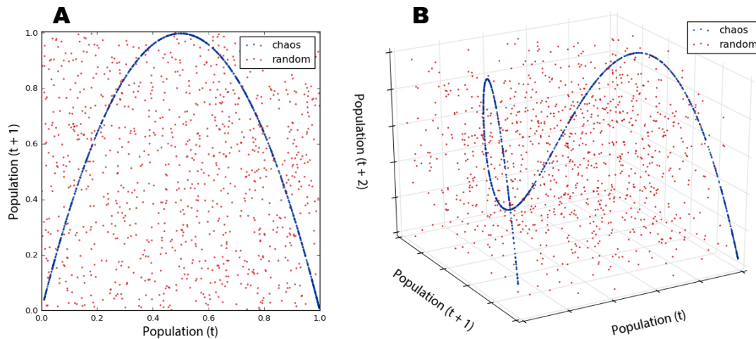
Figure 2.10. Phase diagrams of the time series in Figure 2.9. 10B is a three-dimensional state space version of the two-dimensional 10A.
