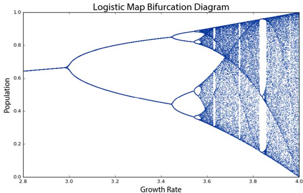
Figure 2.3. Bifurcation diagram of 100 generations of the logistic map for 1,000 growth rate parameter values between 2.8 and 4. The vertical slice above each growth rate depicts the system's attractor at that rate.
