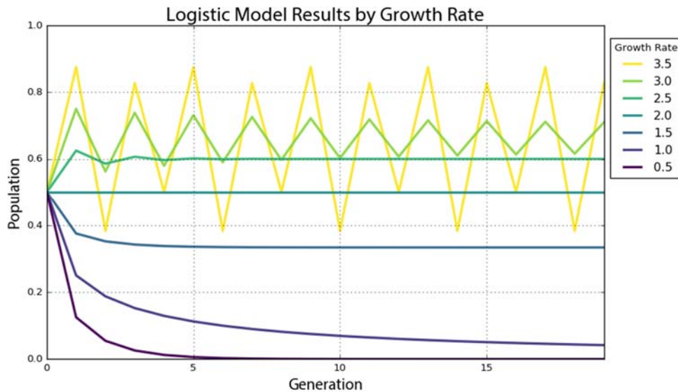
Figure 2.1. Time series graph of the logistic map with 7 growth rate parameter values over 20 generations.
