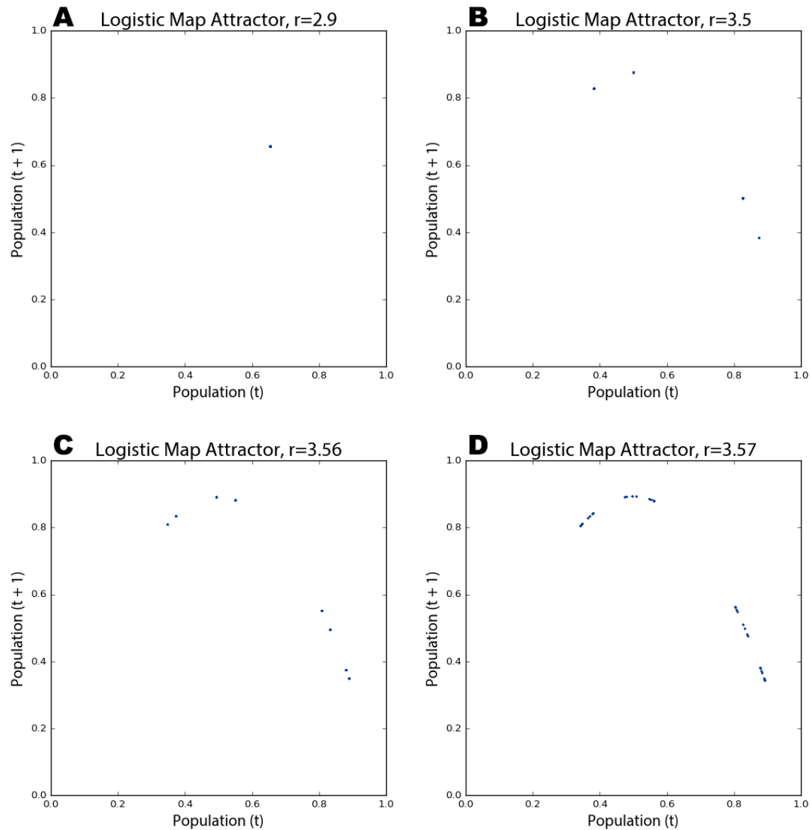
Figure 2.6. Phase diagrams of the logistic map over 200 generations for growth rate parameter values of 2.9 (A), 3.5 (B), 3.56 (C), and 3.57 (D). When the parameter is set to 2.9, the model converges at a single fixed-point. When the parameter is set to 3.5 or higher, the model oscillates over four points, then eight, and on and on as it bifurcates.
