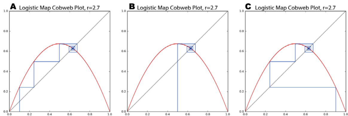
Figure 2.12. Cobweb plots of the logistic map pulling initial population values of 0.1 (A), 0.5 (B), and 0.9 (C) into the same fixed-point attractor over time. At this growth rate parameter value of 2.7, the Lyapunov exponent is negative.
