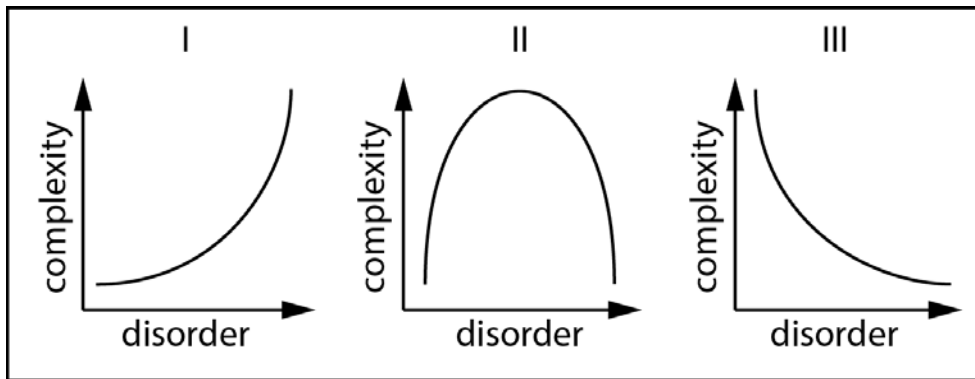
Figure 4.1. Three different categories of complexity. Category I increases monotonically with disorder. Category II is convex, peaking at a midpoint between order and disorder. Category III decreases monotonically as disorder increases. Adapted from Shiner et al. (1999).
