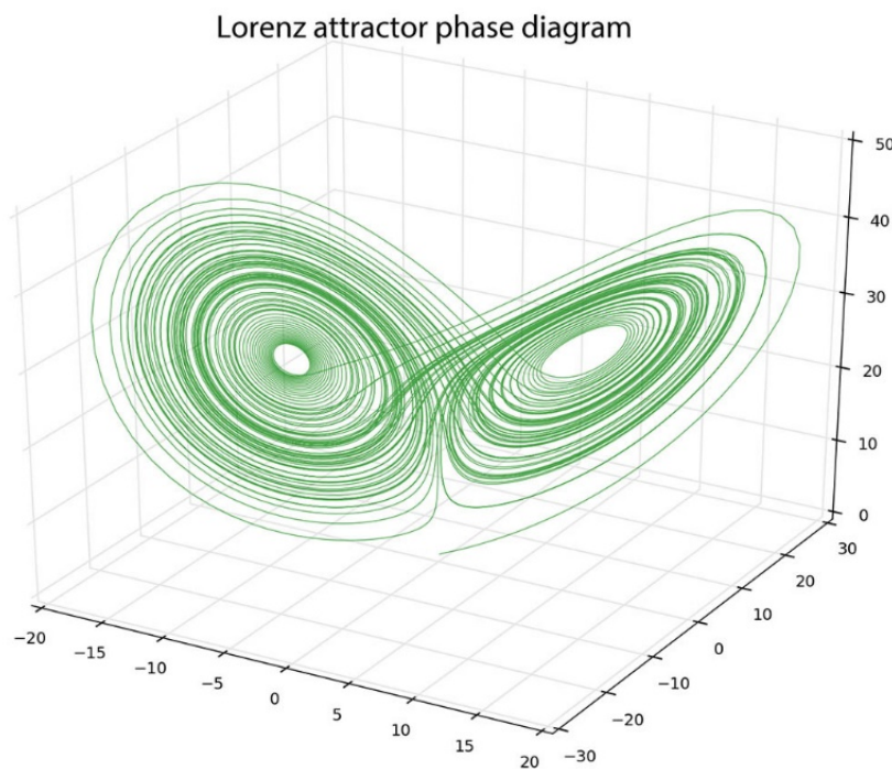
Figure 3.1. An example phase space diagram of the evolution of the Lorenz system over time.
