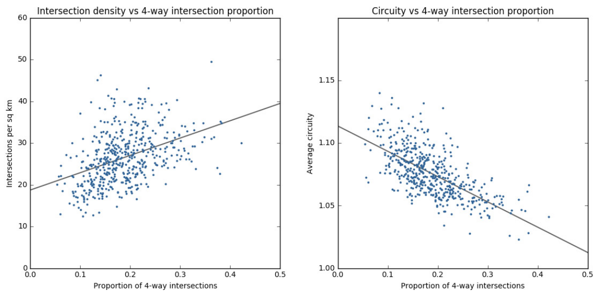
Figure 7.4. Scatterplots of intersection density versus 4-way intersection proportion (left) and average circuitry versus 4-way intersection proportion (right), with simple regression lines to indicate the trend.
