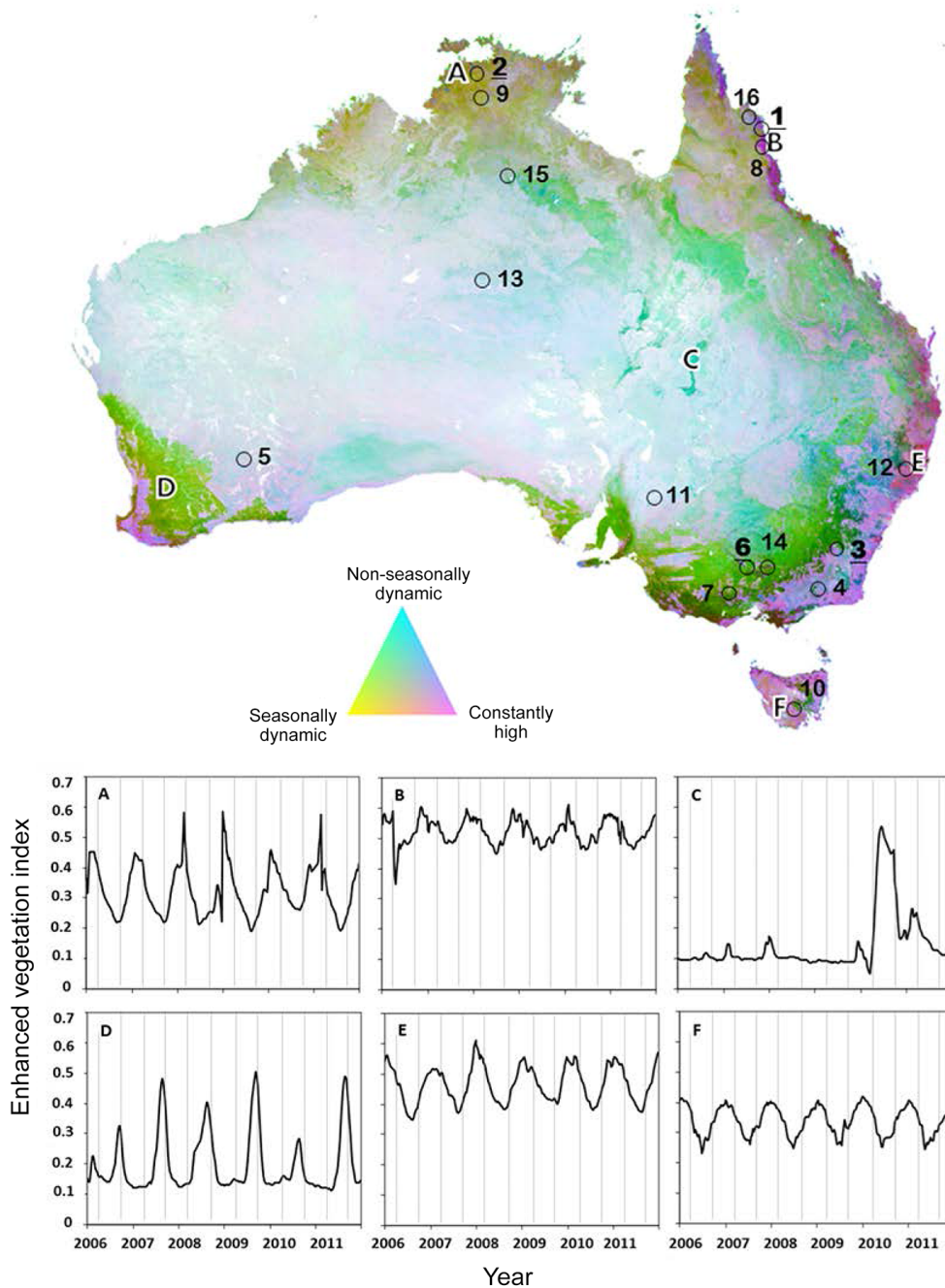
Figure 2. Enhanced vegetation index (EVI) map of Australia obtained from MODIS global 0.05° 8-day reflectance composites for 2000–2012 (MOD09) with a selection of six pixels to demonstrate the following. Yellow areas have a strong seasonal cycle, such as Howard Springs at point A. Cyan areas have relatively strong but non-seasonal variations in EVI, such as Channel Country at point C. Magenta areas have a more constant moderate to high EVI with less temporal variability compared with other sites, which include sites such as Cape Tribulation at point B, the central coast at point E and the Tasmanian highlands at point F. Green areas have both seasonal and non-seasonal variation, such as the wheat belt of Western Australia at point D. Blue areas have relatively high greenness but strong non-seasonal variation. The SD in seasonally adjusted anomalies (yellow) was scaled from 0 to 0.1; SD in mean seasonal cycle (cyan) from 0 to 0.1; and mean EVI (magenta) from 0 to 0.6. Also included are the locations (and Fluxnet codes where applicable) of currently operating phenocams in Australia. Numbers refer to 1. Cow Bay (AU-Cow); 2. Howard Springs (AU-How); 3. Tumbarumba (AU-Tum); 4. Karawatha; 5. Great Western Woodlands (AU-GWW); 6. Whroo (AU-Whr); 7. Wombat (AU-Wom); 8. Robson Creek (AU-Rob); 9. Litchfield (AU-Lit); 10. Warra (AU-Wrr); 11. Calperum (AU-Cpr); 12. Cumberland Plain (AU-Cum) and EucFACE; 13. Alice Springs (AU-ASM); 14. Riggs Creek (AU-Rig); 15. Sturt Plains (AU-Stp); 16. Cape Tribulation (AU-Ctr). Phenocam data used in this paper are from sites 1, 2, 3, and 6.
