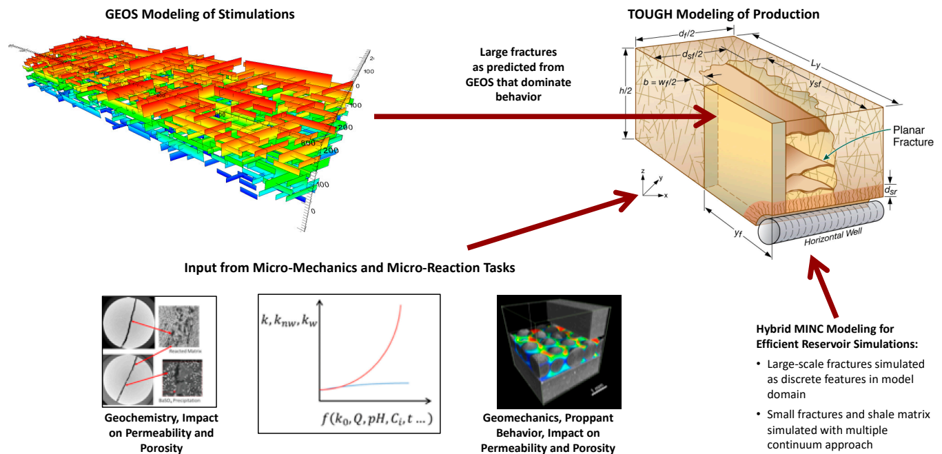
Figure 1. Schematic showing the framework for reservoir-scale stimulation and production simulations informed by micro-scale processes.
