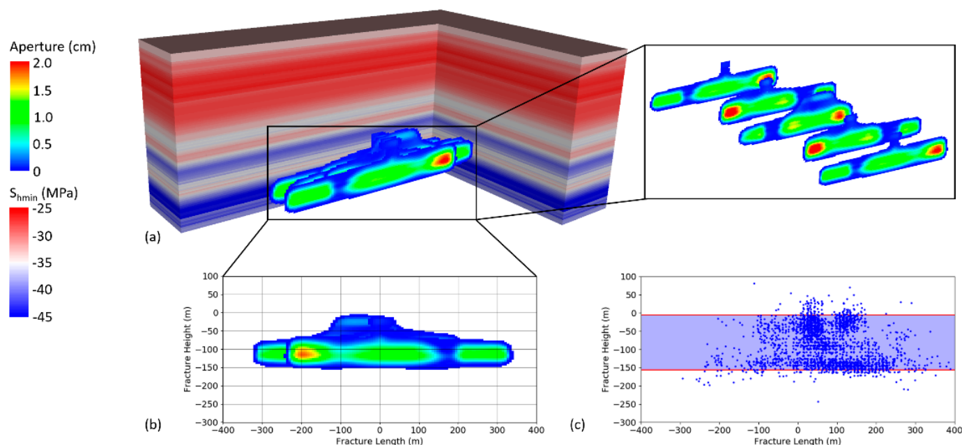
Figure 6. GEOS simulation results and microseismic data. (a) Fracture aperture and minimum horizontal stress distributions; (b) simulated fracture geometry and aperture, front view; (c) fracture extent indicated by microseismic event distributions.
