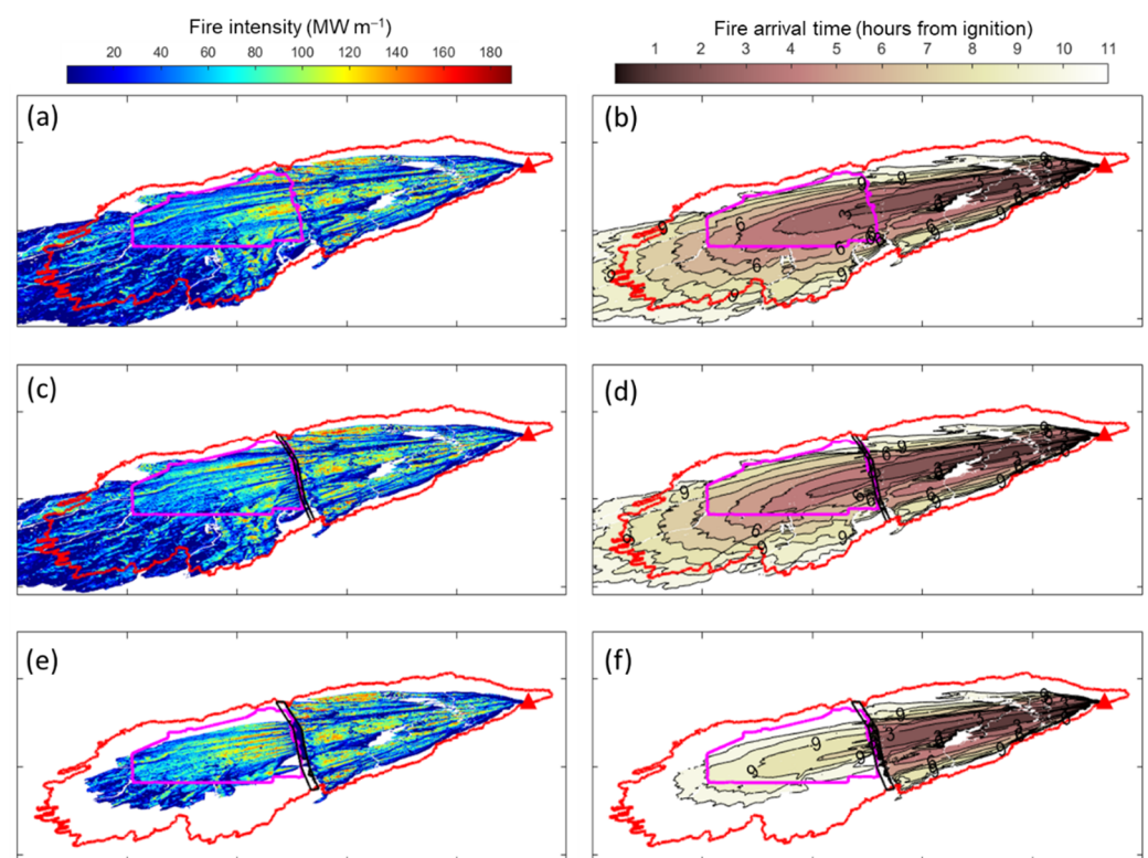
Figure 3. Simulated fire intensity (left) and fire arrival time in hours after 06:30 PST ignition (right) for the verification simulation (a,b), 200 m-wide (c,d) and 400 m-wide (e,f) WUI fuel break scenarios. The locations of the 2018 Camp Fire ignition and WUI fuel break are indicated with a red triangle and black polygon, respectively. Observed burn perimeter at 18:00 PST on 8 November is shown using a red polygon. The Paradise Township boundary is shown with a magenta polygon. In panels (a,c,e), the color bar represents fire intensity with warmer colors corresponding to higher intensities. In panels (b,d,f), the colors correspond to fire arrival times in hours since 06:30 PST, with darker colors corresponding to earlier arrival times.
