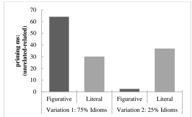
Figure 1: Priming effects (in ms).
