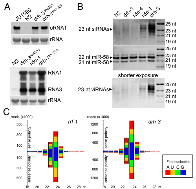
Fig. 4. DRH-3 regulates antiviral RNAi by a mechanism distinct from DRH-1. (A, Upper) Accumulation of Orsay virus RNA1 detected by Northern blot in JU1580, wild-type N2 worms, and genetic mutants defective in drh-3 or drh-1 , as indicated. (Lower) Accumulation of FR1gfp transcripts detected by Northern blot in wild-type N2 worms and genetic mutants defective in drh-3 , rde-1 , or drh-1 , as indicated. (B) Accumulation of FR1gfp-derived siRNAs detected by Northern blot in different genetic backgrounds, as indicated. (Lower) Shorter-exposure image of the same blot. (C) Primary and secondary FR1gfp-derived siRNA populations in rrf-1 and drh-3 mutants. The reads are grouped based on polarity and according to length and the identity of the first nucleotide.
