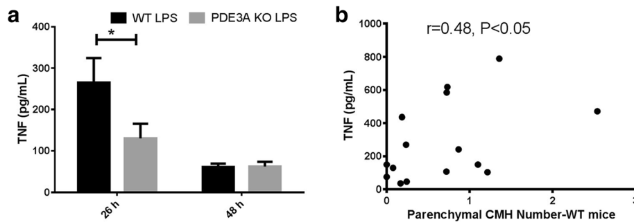
Fig. 4 Significant increase in serum TNF- \alpha levels in LPS-treated WT mice compared with LPS-treated PDE3A KO mice, 26 h after the first LPS injection (or 2 h after the last LPS injection) (a). No significant difference in the serum TNF- \alpha levels between the LPS-treated WT mice compared with the LPS-treated PDE3A KO mice, 48 h after the first LPS injection (a). No detectable TNF- \alpha levels were observed in the saline-treated WT and PDE3A KO mice. Significant correlation between the serum TNF- \alpha levels of LPS-treated WT mice and number of H&E-positive CMH ( N = 15 ) (b). Data are presented as mean \pm SEM (a) and scatter plot with Spearman correlation coefficient (b). Statistical test: Student's t test for TNF- \alpha level comparison at 26 h and Spearman correlation coefficient. * p < 0.05
