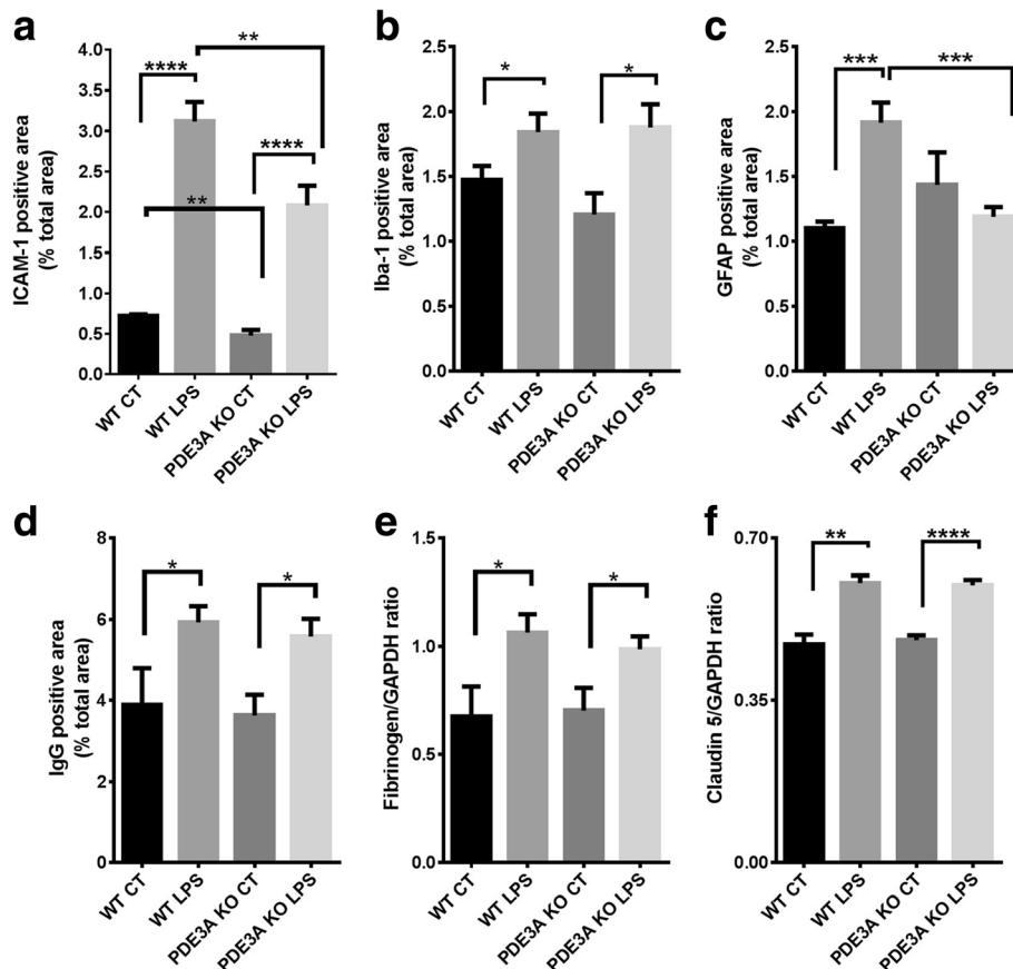
Fig. 7 Effect of genetic deletion of PDE3A on neuroinflammation and BBB function in the inflammation-induced CMH mouse model. Significant increase in ICAM-1 (a), Iba-1 (b), and GFAP (c) positive immunoreactive area in the LPS-treated WT and LPS-treated PDE3A KO mice compared with their respective saline controls. Significant reduction in ICAM-1 in both the saline-treated PDE3A KO and LPS-treated PDE3A KO mice compared with their respective WT controls (a). Significant reduction in GFAP positive immunoreactive area in the LPS-treated PDE3A KO mice compared with LPS-treated WT mice (c). No effect of PDE3A deletion on Iba-1. Significant increase in brain IgG (d), fibrinogen (e), and claudin-5 (f) in the LPS-treated WT and LPS-treated PDE3A KO mice compared with their respective saline controls. No significant difference in any of these markers of BBB function with PDE3A deletion. Data are presented as mean \pm SEM. Statistical test: one-way ANOVA with Bonferroni's post-test or Kruskal-Wallis test with Dunn's post-test. * p < 0.05 , ** p < 0.01 , *** p < 0.001 , **** p < 0.0001
