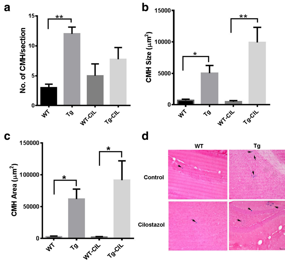
Fig. 5 Pharmacological inhibition of PDE3A and CAA-associated spontaneous CMH development. Significant increase in Prussian blue (PB)-positive CMH number (a), size (b), and area (c) in the Tg mice compared with the WT mice. No significant effect of PDE3A inhibition by cilostazol on any of these CMH parameters. Representative images of PB-positive lesions (indicated by arrows) in WT and Tg mice with or without cilostazol treatment (d). Data are presented as mean \pm SEM. Statistical test: one-way ANOVA with Bonferroni's post-test or Kruskal-Wallis test with Dunn's post-test. * p < 0.05 , ** p < 0.01
