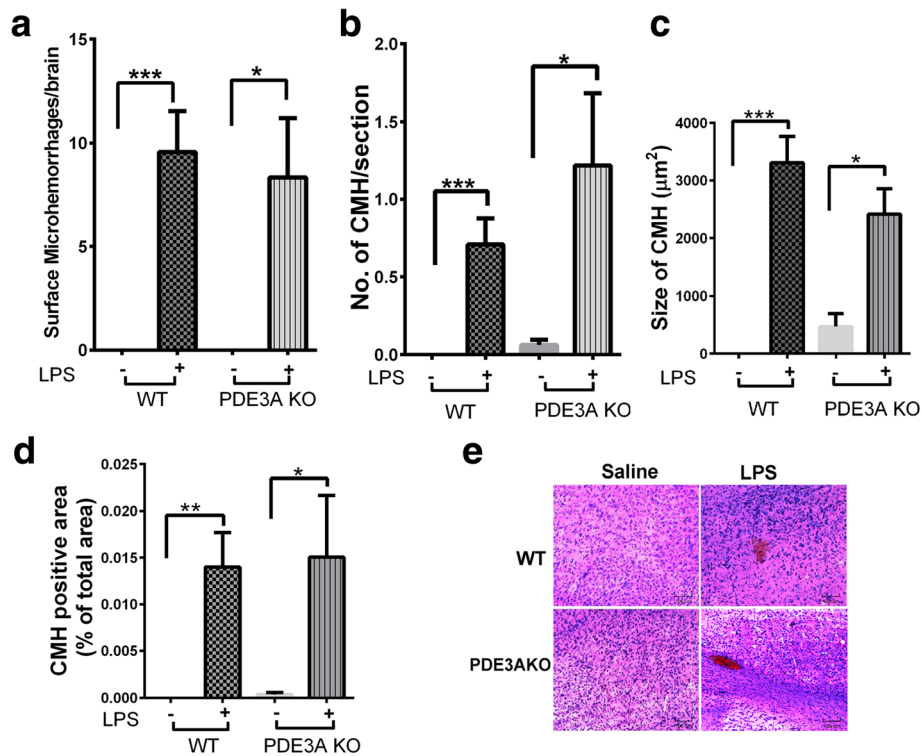
Fig. 3 Genetic deletion of PDE3A and inflammation-induced CMH development: Significant increase in grossly visible surface CMH in the LPS-treated WT and LPS-treated PDE3A KO mice compared with their respective saline controls (a). Significant increase in H&E-positive parenchymal CMH number (b), size (c), and area (d) in the LPS-treated WT and LPS-treated PDE3A KO mice compared with their respective saline controls. Representative images of H&E-positive CMH in saline- and LPS-treated WT and PDE3A -/- KO mice (e). Data are presented as mean ± SEM. Statistical test: one-way ANOVA with Bonferroni's post-test or Kruskal-Wallis test with Dunn's post-test for parenchymal CMH and one-sample t test with a hypothesized mean = 0 for surface CMH. * p < 0.05, ** p < 0.01, *** p < 0.001
