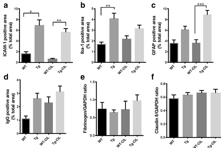
Fig. 8 Effect of pharmacological inhibition of PDE3A on neuroinflammation and BBB function in the CAA-associated CMH mouse model. Significant increase in ICAM-1 (a) and Iba-1 (b) positive immunoreactive area in the Tg mice compared with the WT mice. No effect of PDE3A inhibition with cilostazol on ICAM-1 and Iba-1. Significant increase in GFAP positive immunoreactive area in the Tg mice treated with cilostazol compared with treated WT mice (c). No significant difference in brain IgG (d), fibrinogen (e), and claudin-5 (f) between Tg and WT mice. Pharmacological inhibition of PDE3A had no effect on any of these markers of BBB function. Data are presented as mean \pm SEM. Statistical test: one-way ANOVA with Bonferroni's post-test or Kruskal-Wallis test with Dunn's post-test. * p < 0.05 , ** p < 0.01 , *** p < 0.001
