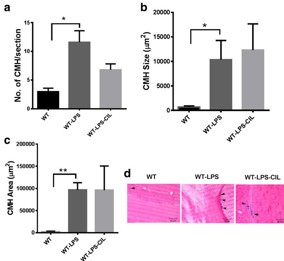
Fig. 6 Pharmacological inhibition of PDE3A and inflammation-induced CMH development. Significant increase in LPS-induced PB-positive CMH number (a), size (b), and area (c) in the WT mice compared with PBS controls. Representative images of PB-positive lesions (indicated by arrows) in WT controls, mice treated with LPS or with LPS and cilostazol (d). No effect of cilostazol treatment on any of these CMH parameters. Data are presented as mean \pm SEM. Statistical test: one-way ANOVA with Bonferroni's post-test or Kruskal-Wallis test with Dunn's post-test. * p < 0.05 , ** p < 0.01
