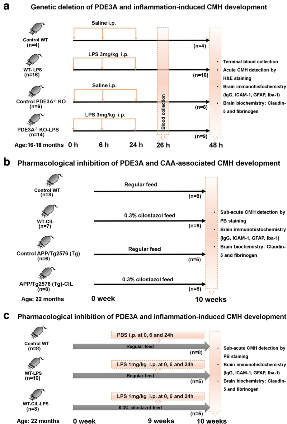
Fig. 1 Experimental designs used in the current study. Workflow and treatment groups used to determine the effect of genetic deletion of PDE3A on inflammation-induced CMH development (a), pharmacological inhibition of PDE3A with cilostazol on CAA-associated spontaneous CMH development (b), and pharmacological inhibition of PDE3A with cilostazol on inflammation-induced CMH development (c)
