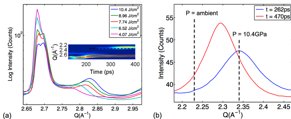
Figure 2. (a) Fluence dependence of aluminum (111) reflection at maximum compression. Inset: Zoom diffractiongram of aluminum and rocksalt dynamics shown as a function of momentum transfer and time. (b) Q -dependence of shock-induced rocksalt reflection shown at t = 262 ps (blue) and at t = 470 ps (red) showing maximum deflection of peak and subsequent relaxation toward ambient pressure.
