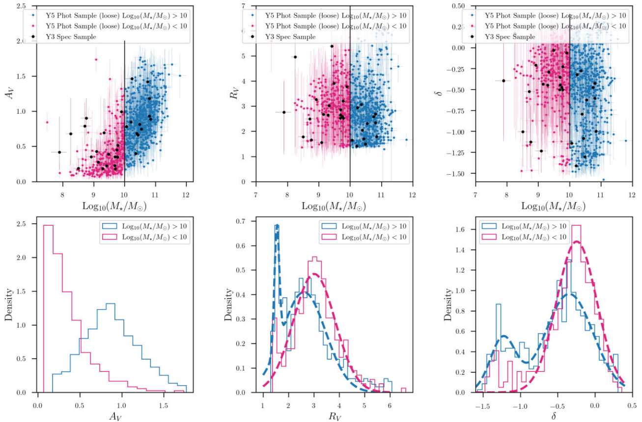
Figure 3. Top: dust parameters A_V , R_V (as defined in equation 5), and \delta estimates from this work as a function of stellar mass, derived using a lognormal SFH. Blue points represent galaxies whose photometry data are found in the DES Year 5 sample (Y5 Phot Sample loose), black points are those galaxies found in the DES Year 3 spectroscopic Sample. In all cases, we use three of the SN fields. In all six plots, galaxies that did not meet a \chi^2 cut are not shown and are not used in calculation of fits. The vertical line denotes the location of the 10^{10} M_\odot split. The error bars show the 16th and 84th percentile around the median using the posterior distributions from BAGPIPES. Bottom: distributions of A_V , R_V , and \delta values above and below the 10^{10} M_\odot split, the location of the observed mass step. For the R_V and \delta distributions, we include Gaussian curves to highlight the distributions' dependence on mass.
