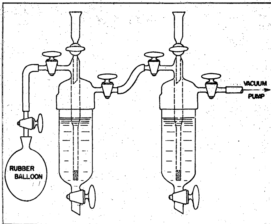
APPARATUS FOR CARBON DIOXIDE ABSORPTION
