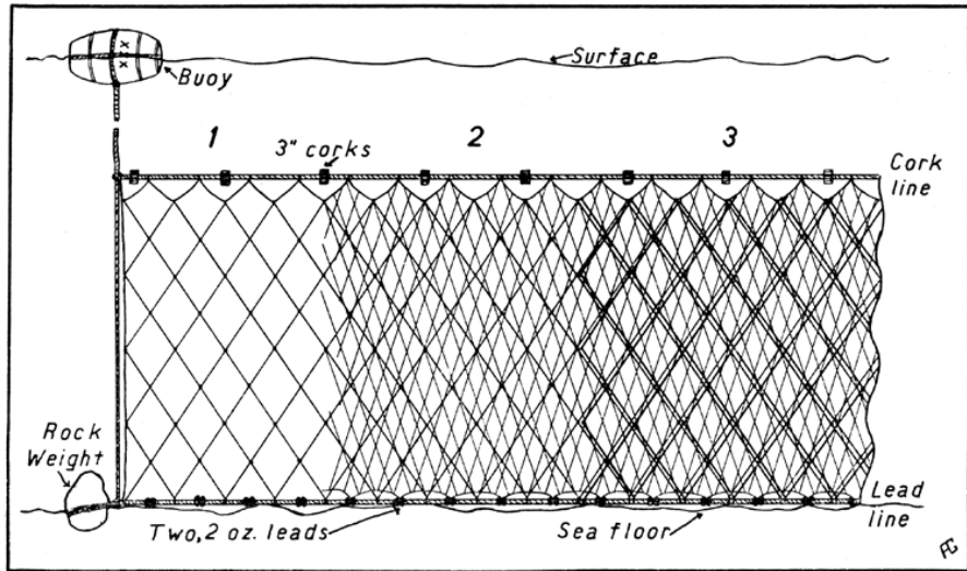
FIG. 7. Diagrammatic drawing of a set trammel net. (1) Shows one of the guard mesh, (2) one guard mesh and the smaller inner webbing, (3) both guard meshes and the inner net in place.
