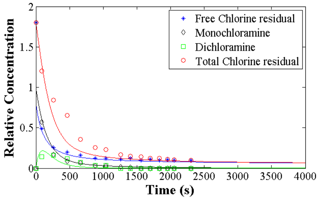
Figure 4-9 Experimental data and simulation results in batch reactor at pH=7, T=15°C, Cl/N=1.8
