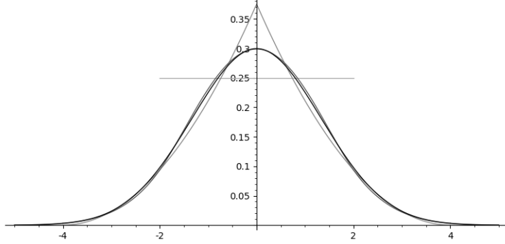
Figure 3: Isogeny Sato-Tate distribution for g \leq 4 .
