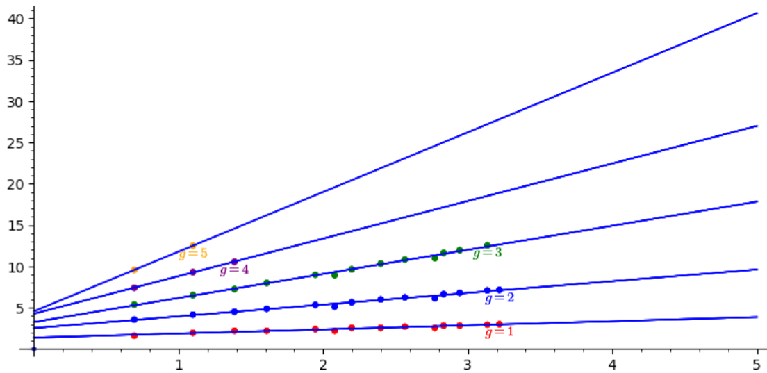
Figure 1: Plots of (\log q, \log N(g, q)) for each g and q \leq 27 in the database. The least square values of \log N(g, q) = a \log q + b are given in Table 3.
