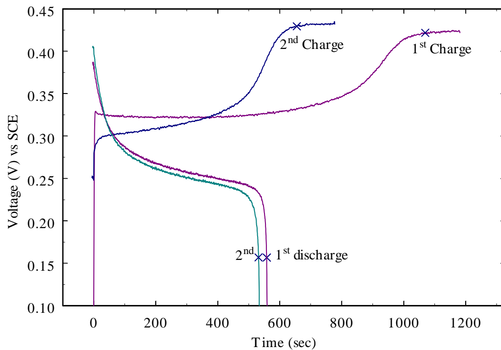
Figure 2. First two constant current (0.1 mA) charge/discharges for a 70 \mu\text{g} nickel hydroxide film. The x represents the point where the electrode is fully charged or discharged; these endpoints were used in the generation of Figure 3.
