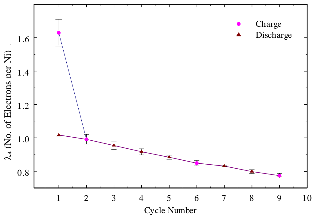
Figure 4. Number of electrons transferred per Ni during charge and discharge of a 70 \mu\text{g} nickel hydroxide film. The charge/discharge values from Figure 3 have been corrected for the oxygen evolution reaction as described in the text. The values plotted are an average of 3-4 data sets, and the error bars represent the spread in the data.
