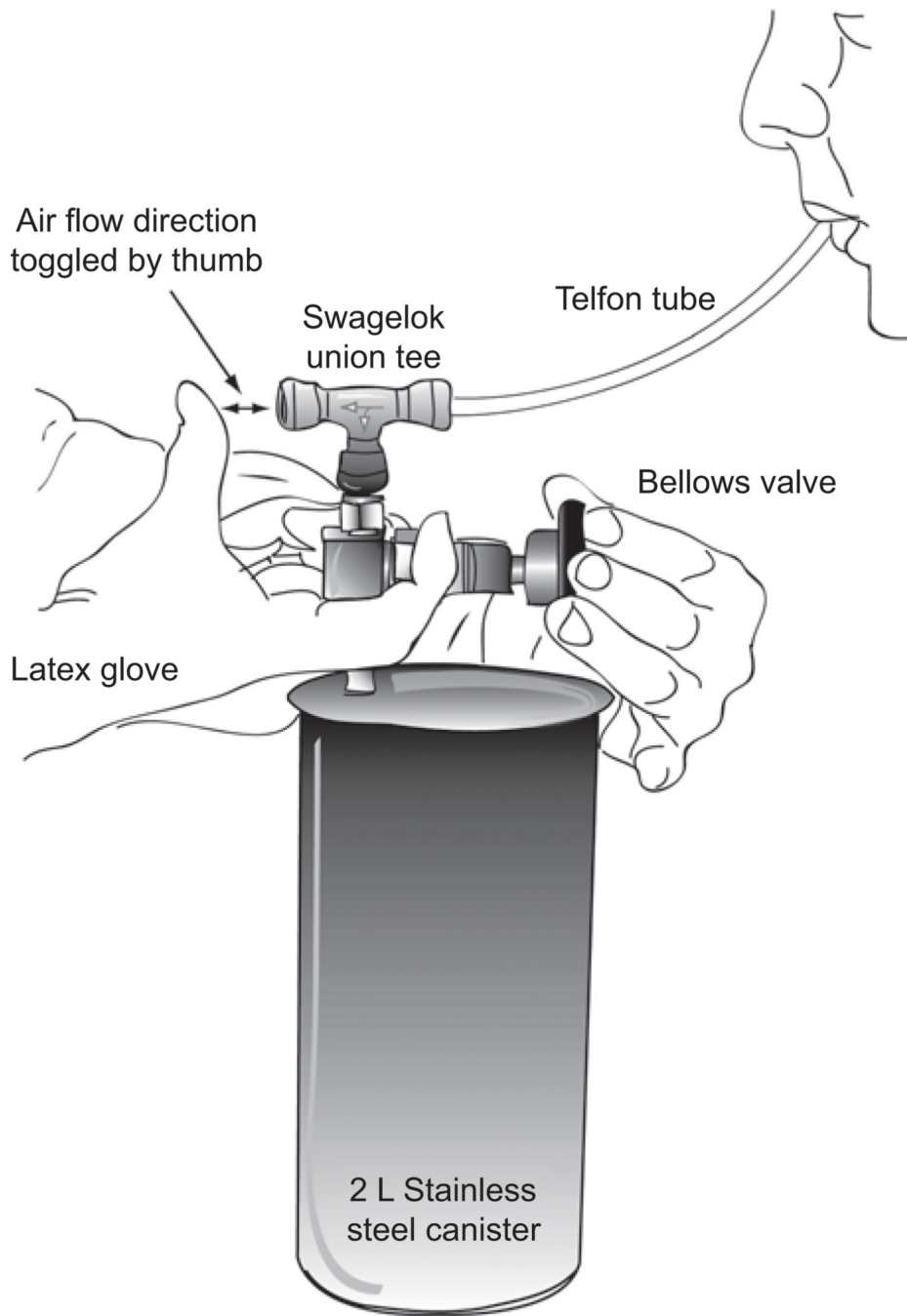
Figure 1. Diagram of a hydrocarbon/CO 2 breath sampling apparatus.
