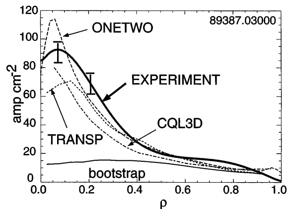
FIG. 2. The profile of measured noninductive current profile compared to various theoretical models of neutral beams current drive. The noninductive current is the combination of neutral beam driven and bootstrap driven currents; the theoretical estimate of the bootstrap portion is shown for reference.
