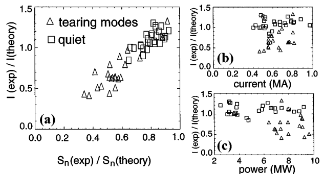
FIG. 4. Driven current discrepancy versus (a) neutron discrepancy, (b) plasma current, (c) neutral beam power. I_{\text{exp}} is the integral of noninductive current measured inside \rho > 0.35 , and I_{\text{theory}} is the same quantity predicted by the transport code ONETWO. S_n(\text{exp})/S_n(\text{theory}) is the ratio of the total measured neutron rate to the predicted neutron rate using the same fast ion model as for the current drive estimation. Each data point represents a 1 sec long average of the experiment and a 1 sec transport simulation. \triangle represents tearing fluctuations observed on external Mirnov coils; \square , no measurable fluctuations observed on external Mirnov coils (small signals may be seen on ECE).
