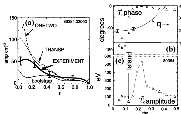
FIG. 3. (a) The same as Fig. 2, but for a case with a tearing mode at 22 kHz. Magnetics indicates that the mode is m/n = 2/1 and is stationary in the rest frame of the rotating plasma. (b) The phase of the perturbation indicates an inversion at \rho = 0.12 corresponding to q = 2 . (c) The amplitude of coherent perturbation of the electrons temperature from the tearing mode. Note that the maximum perturbation is near the outer edge of the island as expected.
