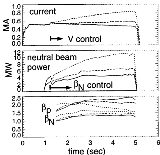
FIG. 1. Time histories of plasma current, neutral beam power, \beta_N , and \beta_p for representative discharges with \beta_N = 1.4 \pm 0.1 and V_\Omega = 50 (solid), 100 (dashed), and 20 mV (dotted). Feedback control of \beta_N control was implemented by modulating the duty cycle of the neutral beams.
