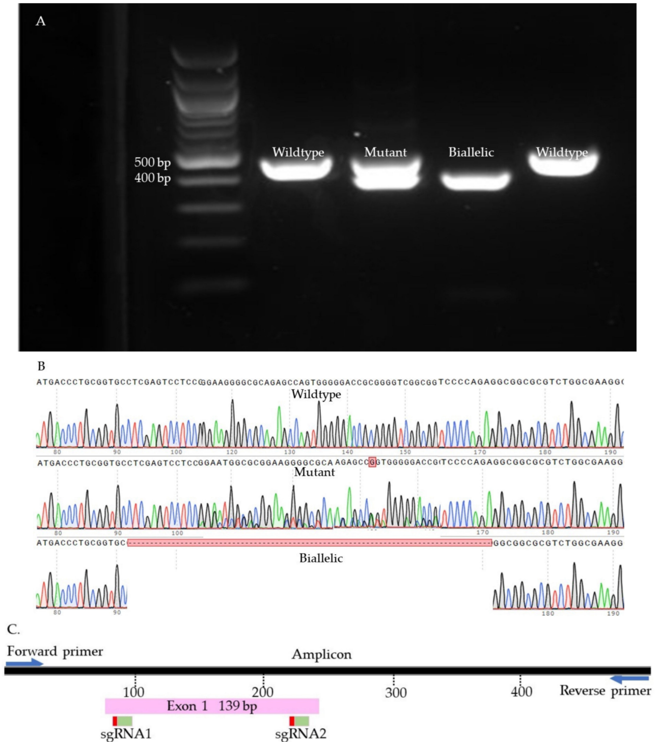
Figure 7. SOCS2 knock-out samples. (A). Gel electrophoresis. (B). Sanger sequences (C). Map of the targeted site.
