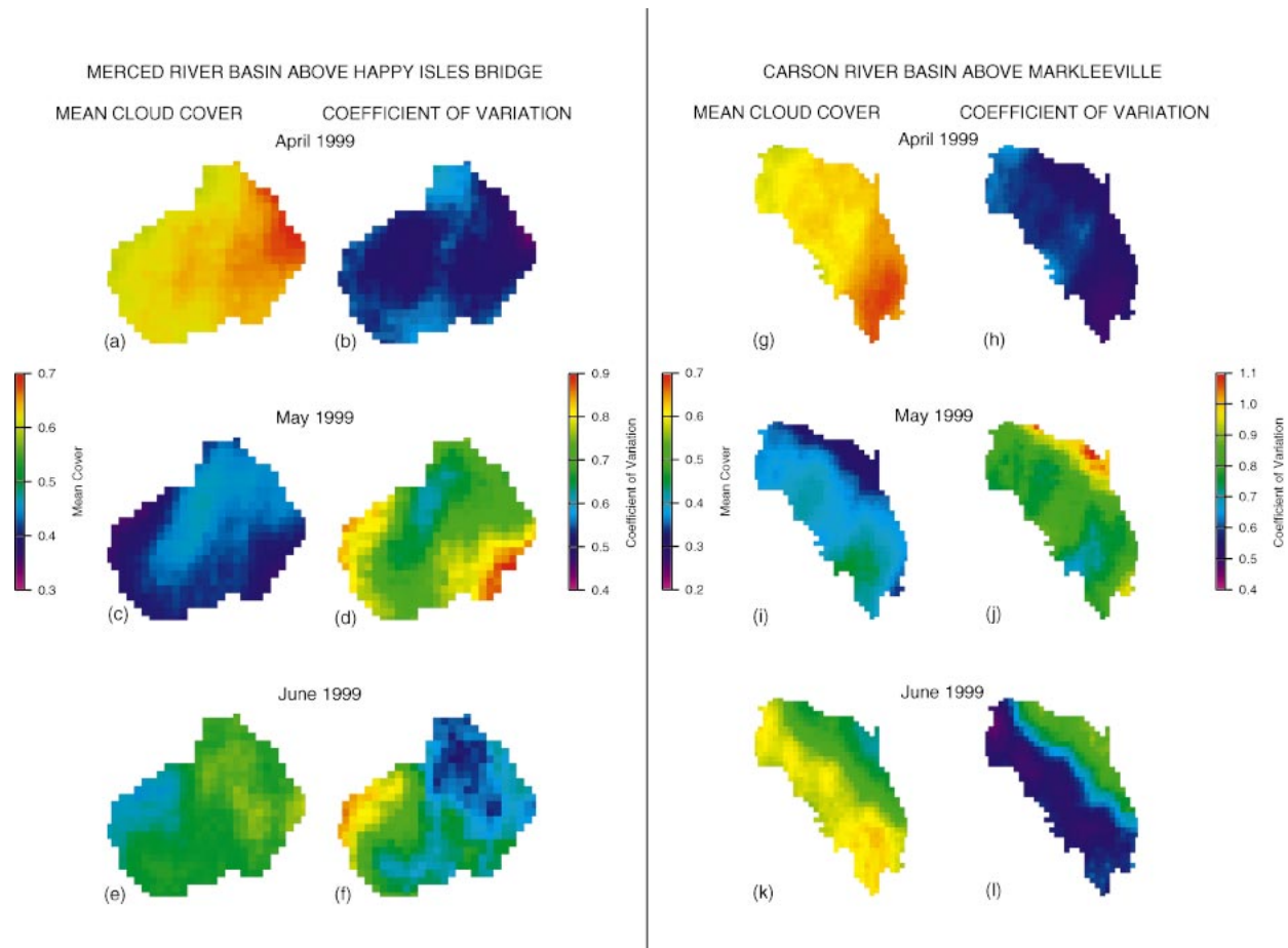
FIG. 5. Mean monthly cloud cover and coefficient of variation (mean/standard deviation) for the months and basins indicated. See Table 2 and the text for details on data used.
