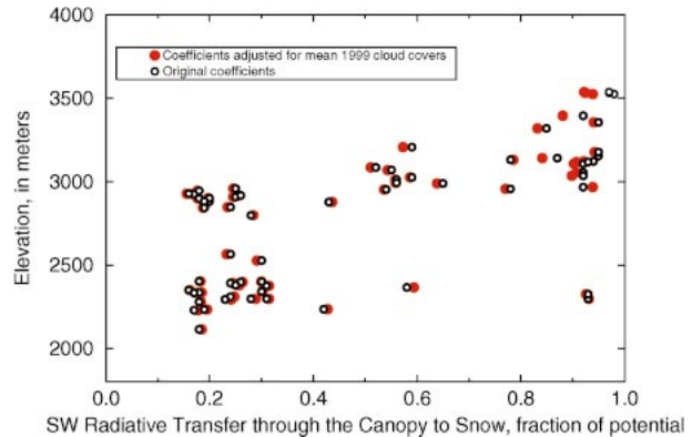
FIG. 12. Relations of shortwave radiative (through plant canopy to snowpack) transfer coefficients to elevation, in the Merced River model (above Happy Isles Bridge), before and after adjustments for seasonal-mean cloud cover, spring 1999.
