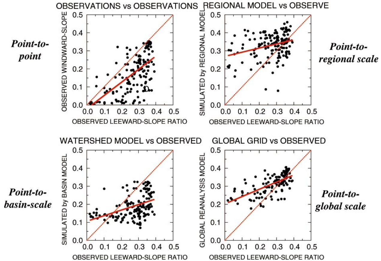
FIG. 8. Ratios of daily insolation rates from various sources around the Sierra Nevada to estimates of the corresponding top-of-atmosphere insolation rates. Windward observations are from the Central Sierra Snow Laboratory, leeward observations are from the Sierra Nevada Aquatic Research Laboratory, regional simulated values are from the Regional Spectral Model (Juang et al. 1997; Dettinger et al. 1999) nested in the National Centers for Environmental Prediction–National Center for Atmospheric Research (NCEP–NCAR) reanalysis fields (Kalnay et al. 1996), watershed model values are from a PRMS model of the American River basin (Jeton et al. 1996), and global values are from the NCEP–NCAR reanalysis.
