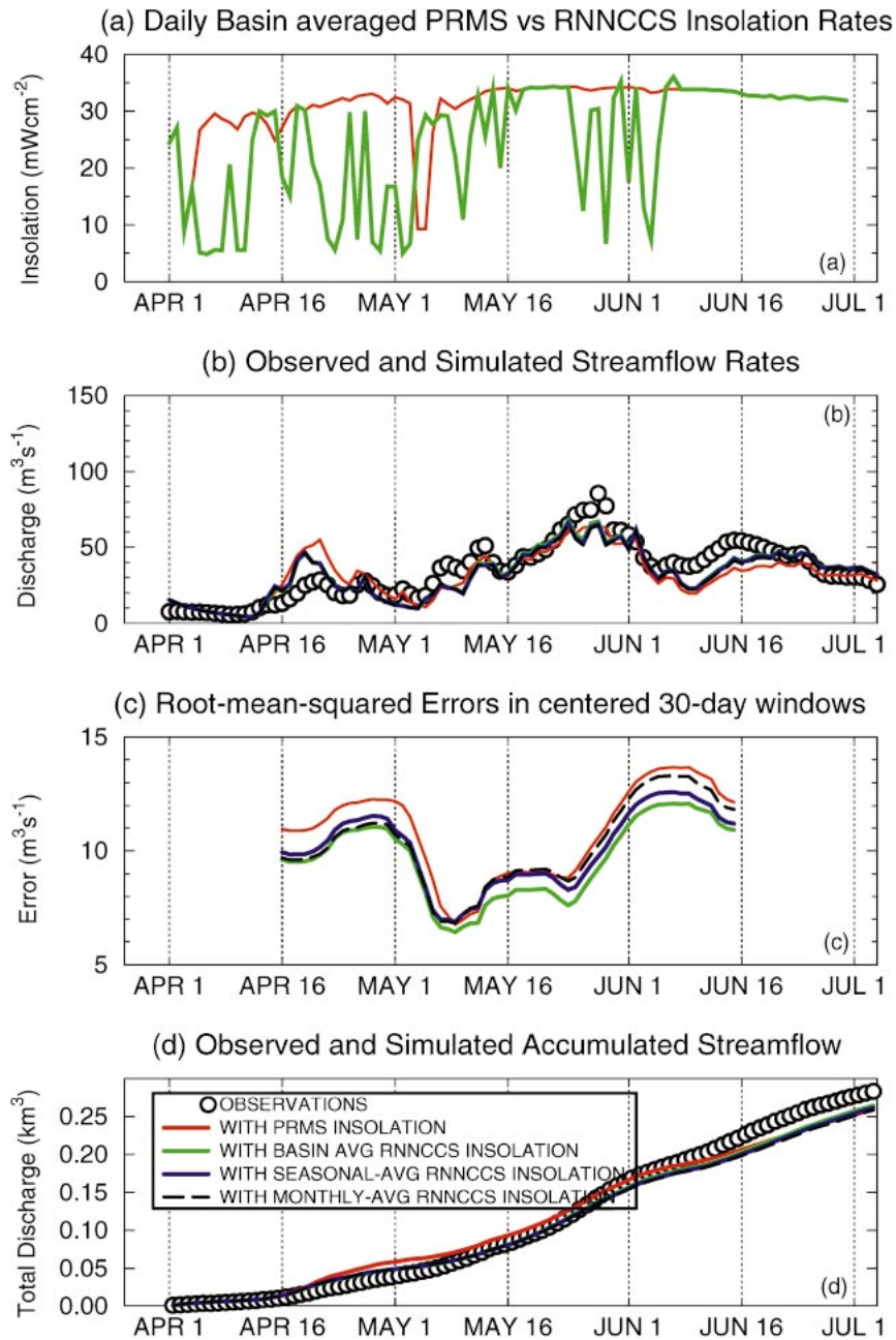
FIG. 14. Same as in Fig. 13 but for the East Fork of the Carson River basin.
