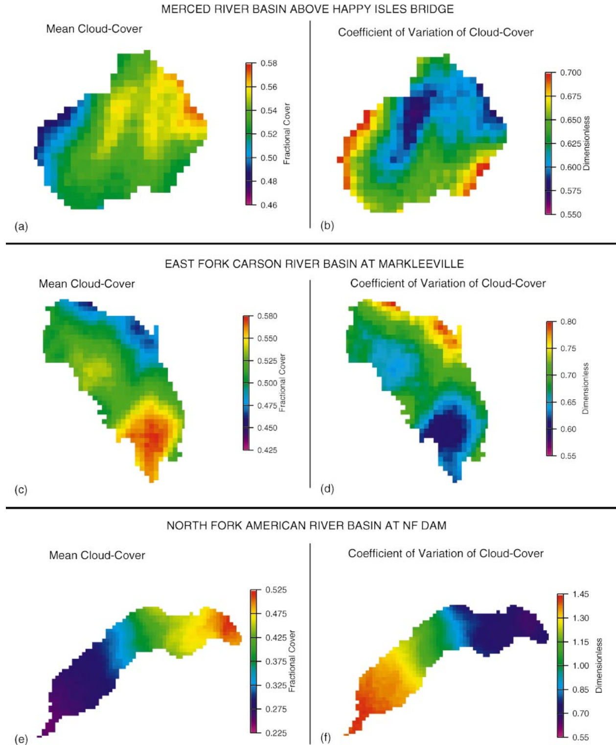
FIG. 6. Analogous to Fig. 5 but for the entire 1999 snowmelt season.
