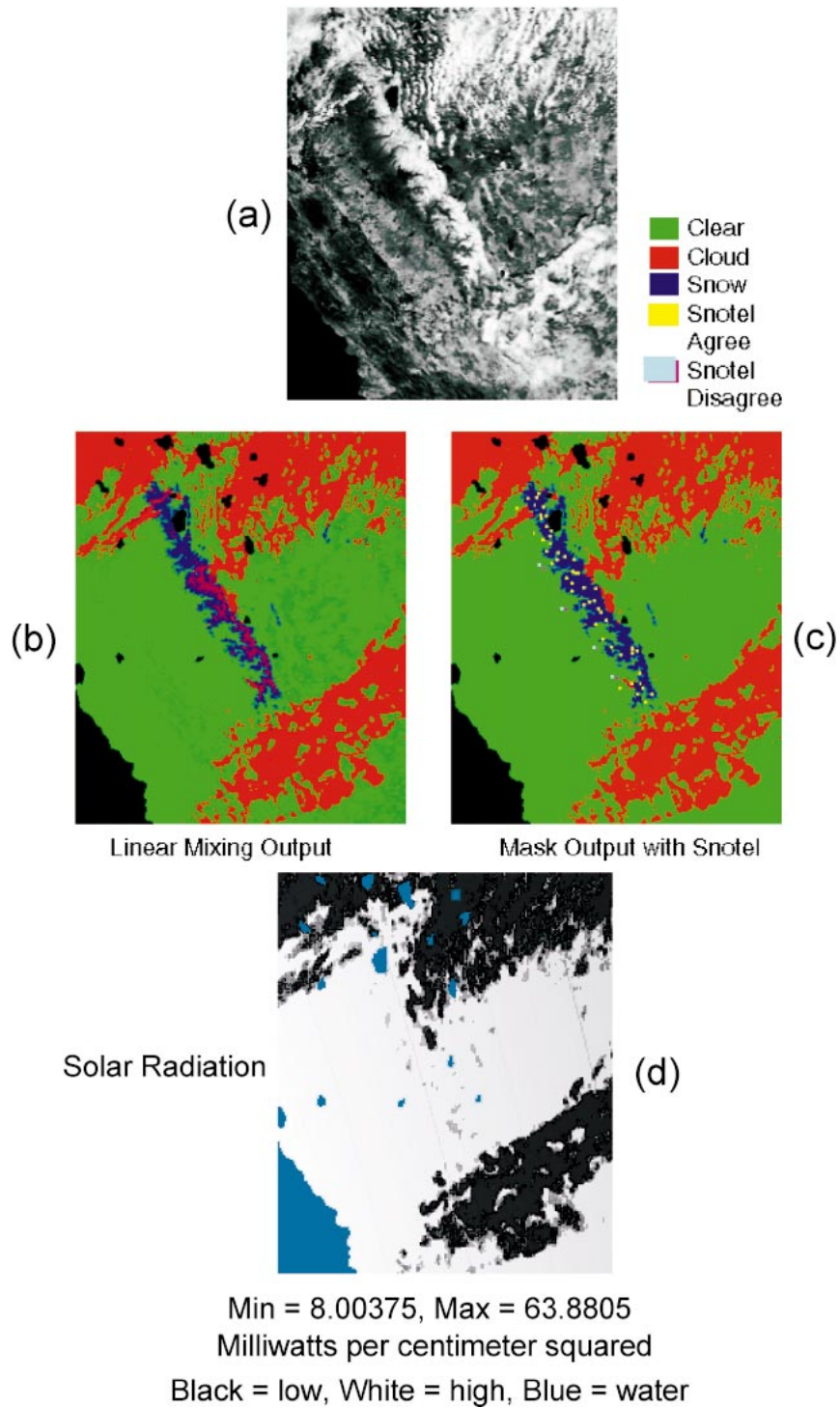
FIG. 3. (a) GOES broadband visible data for 19 Apr 1999. The area imaged corresponds to the dashed box in Fig. 1. (b) The RNNCCS-linear mixing model classification. (c) The RNNCCS discrete classification with snowpack telemetry-instrumented validation (SNOTEL) sites shown. (d) Insolation reaching the ground based on satellite-detected cloud cover. See text for details.
