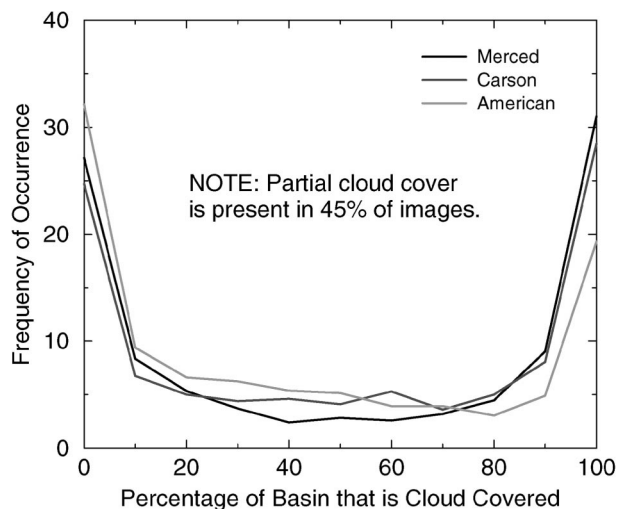
FIG. 10. Analogous to Fig. 9 but for percentage of a given Sierra Nevada river basin area covered by cloud (spring/summer 1999).
