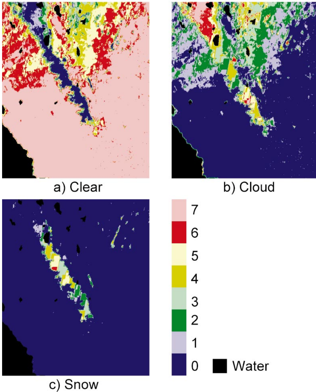
FIG. 7. Two-dimensional frequency diagrams that show the number of times in a day (19 Apr 1999) that a given pixel was a member of a specific class (cloud, snow, or clear land).
