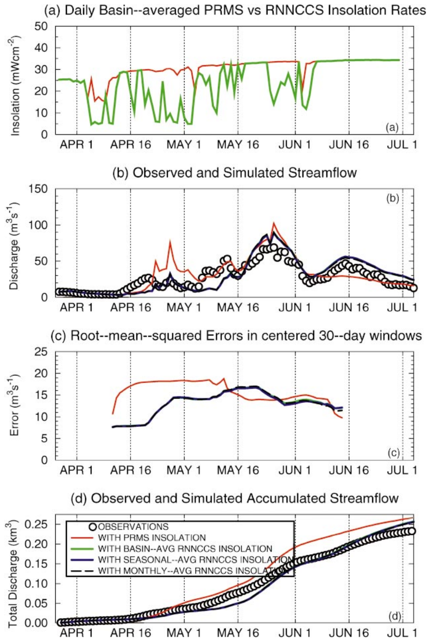
FIG. 13. Comparisons of (a) daily PRMS-estimated and RNNCCS insolation estimates and (b) observed and simulated streamflows, along with (c) rms errors, for Merced River basin at Happy Isles Bridge for the spring snowmelt season 1999. (d) Cumulative volume flow for the different insolation estimates as indicated.
