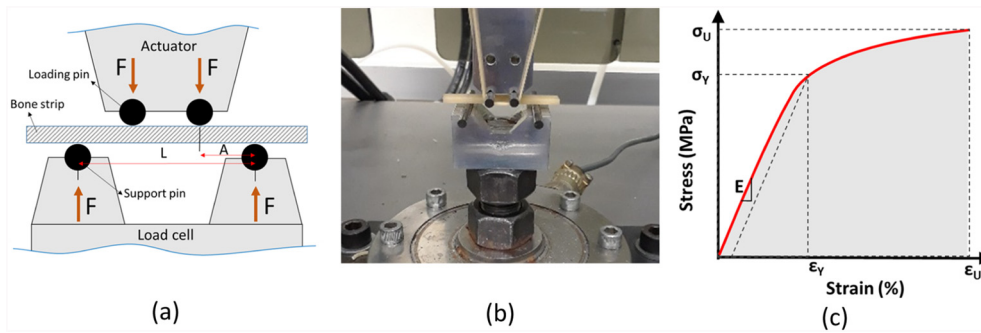
Fig. 1. Standard four-point bending setup to measure the tensile mechanical properties of cortical bone specimens. (a) Schematics of the cross-point bending jigs at the longitudinal cross-section (loading and support pins diameter = 3 mm, L = 24 mm, A = 8 mm; bone strip thickness = approx. 2 mm). The experiments were displacement-controlled at 0.1 mm/s rate when the force was recorded. (b) Prepared bone cortical bone strips (approx. 40 mm length) under mechanical loading using the fabricated four-point bending jigs (aluminum seats and tungsten carbide pins)
