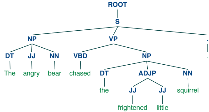
Figure 1: An example of a parse tree for the sentence “The angry bear chased the frightened little squirrel.”
