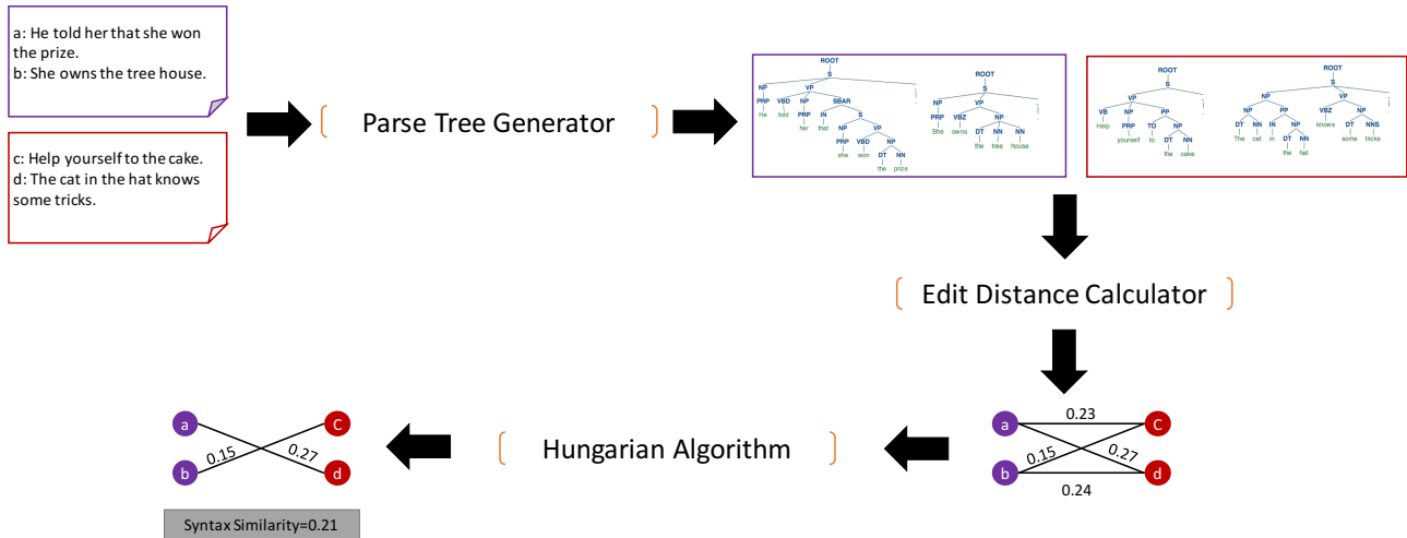
Figure 3: Syntax Similarity Calculation Process. The edit distance calculator module calculates the similarity of each pair of parse trees which are outputted by the parse tree generator module. In the last step, the Hungarian algorithm module finds the minimum weight perfect matching of the graph of sentences’ parse trees. The bold edges are the ones that are selected by the Hungarian algorithm. The overall syntax similarity of the two document is the summation of the selected edges’ weights divided by the number of edges.
