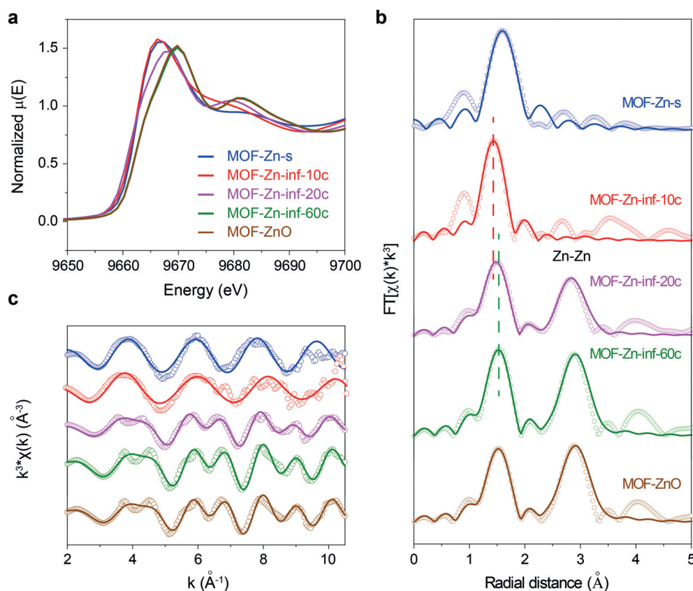
Figure 4. X-ray absorption analysis. a) Normalized Zn K-edge XANES spectra. b) Corresponding EXAFS spectra ( \circ ) and their fitting results ( — ) in R-space. Dashed lines indicate the peak position of Zn-ligand first shell for MOF-Zn-inf-10c and MOF-Zn-inf-60c. c) Corresponding EXAFS spectra ( \circ ) and their fitting results ( — ) in K-space.
