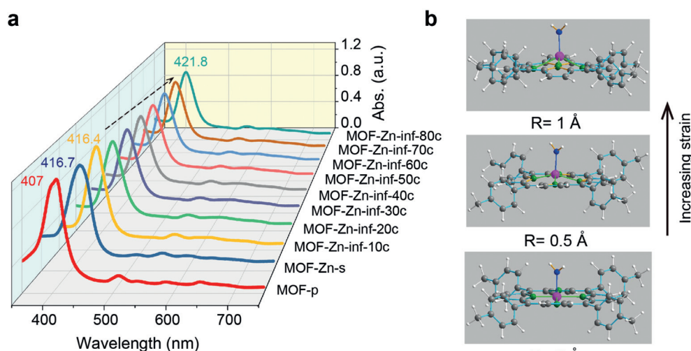
Figure 5. Impact of varied number of VPI cycles on MOF-Zn-inf. a) UV/Vis spectra of MOF-p, MOF-Zn-s, and MOF-Zn-inf with varied number of VPI cycles (0 to 80 cycles). b) DFT-predicted strain in MOF structures (Zn pink, C gray, N green, O blue, H white), correlated to UV/Vis changes provided in the Supporting Information, Table S3. Results demonstrate a gradual strain on the metal–ligand center.
