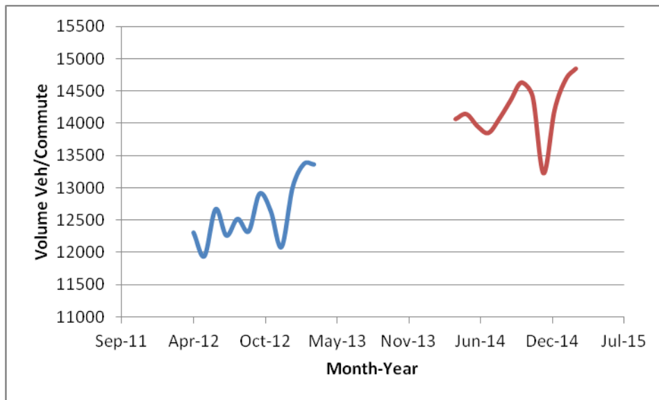
Figure 6: SR 24 WB AM, Average Vehicles Per Commute Period (5:00-10:00) by Month [Standard Commute]
