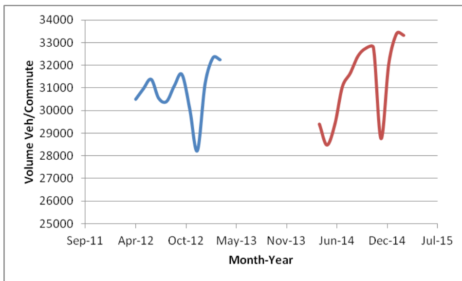
Figure 7: SR 24 EB PM, Average Vehicles Per Commute Period (14:00-20:00) by Month [Standard Commute]
