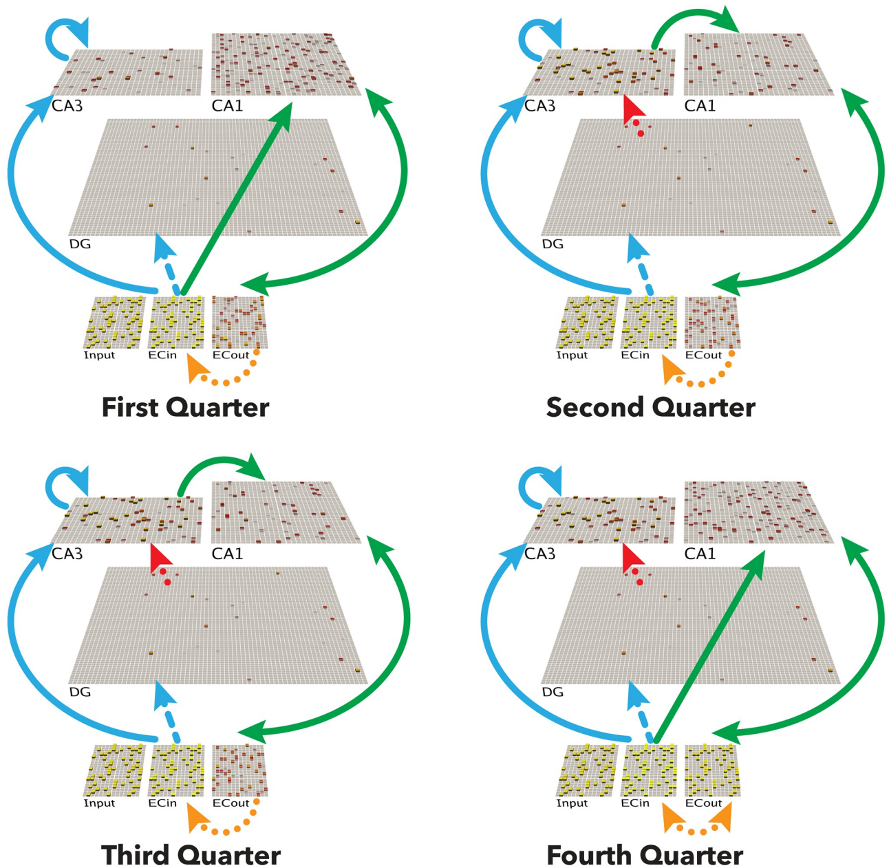
Fig 1. Architecture of the Theremin model. Visual depiction of one full theta-cycle training trial, separated into four different phases within the cycle (i.e., four quarters, each representing 50 ms). The CA1 learns to properly decode the CA3 pattern into the corresponding EC representation, while CA3 learns to encode the EC input in a more pattern-separated manner reflecting DG input. Arrows depict pathways of particular relevance for that quarter. First Quarter: Blue arrows show initial activation of CA3 and DG via monosynaptic pathways from ECin (superficial layers of EC). Green arrows show CA1 likewise being monosynaptically driven from ECin, and in turn driving ECout (deep layers) with bidirectional connectivity. Second Quarter: Red arrow indicates DG driving CA3, providing a target activity state over CA3 relative to the first quarter state. Also, CA3 starts to drive CA1, resulting in full “attempted recall” state over ECout by the end of the Third Quarter . Fourth Quarter: the ECin drives ECout (Orange arrow), which in turn drives any resulting changes in CA1. Note: The fourth quarter is the plus phase for all error-driven learning projections, the second quarter and the third quarter are the minus phase for CA3 → CA1, and the first quarter is the minus phase for ECin → CA1, CA3 → CA3, ECin → CA1, and CA1 ↔ ECout (see Methods for more details). Solid lines represent projections that have error-driven learning + Hebbian learning, dashed lines represent projections that only have Hebbian learning, dotted lines represent projections that do not learn in the model.
