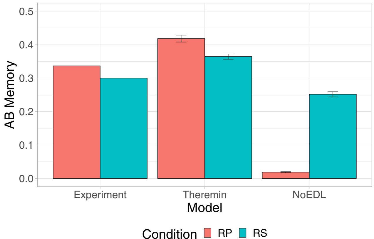
Fig 7. Testing effect simulation. The testing effect refers to memory increase when retrieving learned information, compared to restudying. In the experiment [55], subjects learned 30 Eskimo/English word pairs, went through either retrieval practice (RP) or restudy (RS), and then got a final test. We modeled a similar process using the Theremin model and the NoEDL model (for modeling details, see Methods ). Results show that the Theremin model was able to achieve qualitative fit to the experiment data, while the NoEDL model lost desirable memory performance in RP compared to RS, suggesting that error-driven learning might be crucial to the testing effect.
