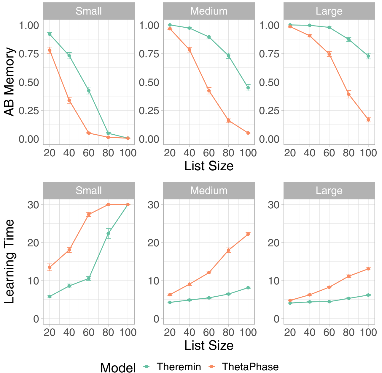
Fig 3. Theremin vs. ThetaPhase on AB memory and learning time for all three network sizes. The Theremin model was better at counteracting interference across all list sizes and network sizes, and had significantly faster training time across all list sizes and network sizes.
