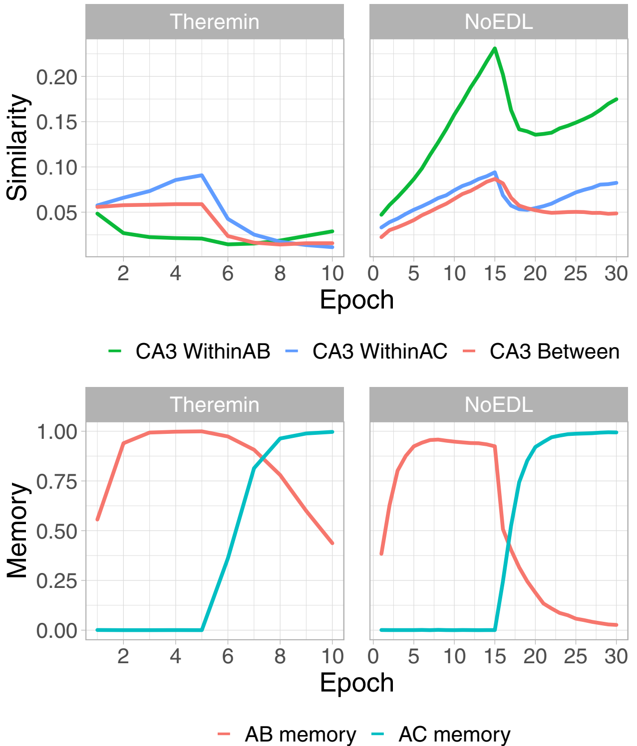
Fig 5. Statistics for area CA3 over the course of testing (List 100, Medium sized network). Representational similarity analyses (RSA) for area CA3 for Theremin vs. NoEDL show how the error-driven learning in Theremin reduces the representational overlap (top left) whereas the Hebbian learning in NoEDL increases the representational overlap (top right). This explains the differential interference as shown in the AB Memory plot for each case (bottom row). The number of epochs used in Theremin training was set to a fixed number (i.e., 10) that enabled complete learning of AB and AC lists, while in NoEDL was set to the maximum amount used in the current paper (i.e., 30).
