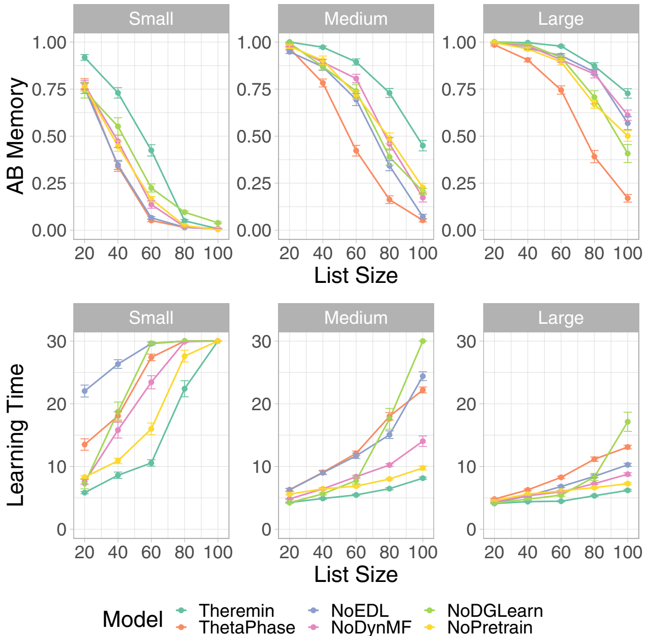
Fig 4. Theremin vs. other models on AB memory and learning time. Theremin and ThetaPhase data are the same as in Fig 3, shown for reference purpose here. NoEDL is the Theremin without the new error-driven learning mechanism. NoDynMF is the Theremin with same mossy fiber strength during training and testing. NoDGLearn is the Theremin with ECin → DG learning off. NoPretrain is the Theremin without pretraining CA1. Each of these factors makes a significant contribution as seen in decrements relative to the full Theremin in interference resistance (AB memory) and learning time.
