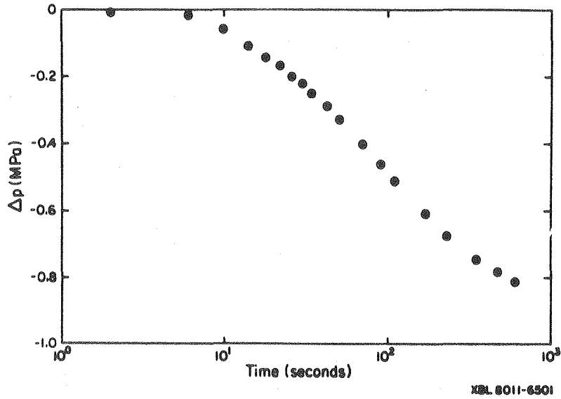
Figure 3a. Generated drawdown pressure.
