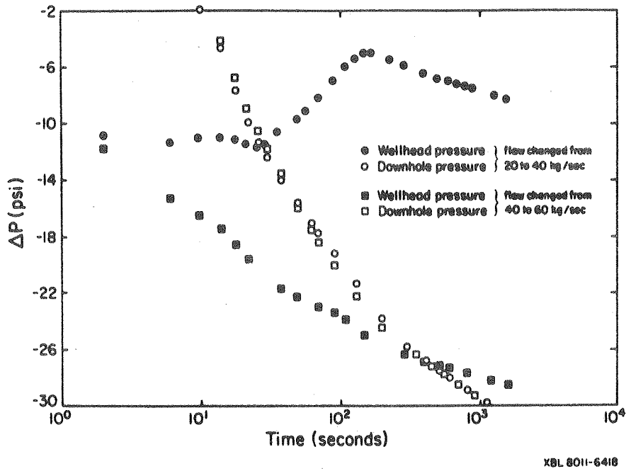
Figure 1. Plot of wellhead and downhole pressure transients for two drawdown tests.
