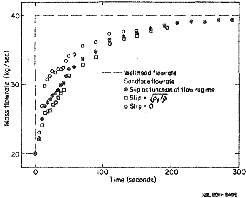
Figure 3b. Calculation of sandface flowrate using different slip correlations.
