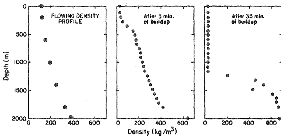
Figure 6. Calculation of density profile in a two phase well during a shut in test.
