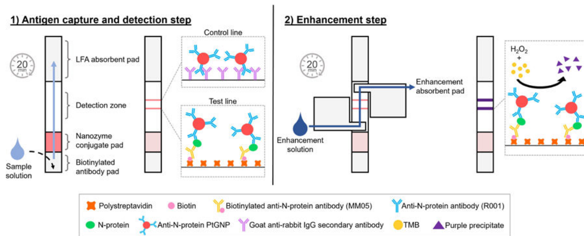
Fig. 5. Simplified schematic of assay steps and paper segments touching the LFA test strip. (1) Sample is applied to the sample well above the test strip where biotinylated antibody and PtGNPs are rehydrated and antigen capture occurs at the detection zone. (2) After pressing the button to move the middle piece of the casing down, enhancement buffer is released to rehydrate the dehydrated enhancement reagents and flow through the test strip resulting in signal enhancement at the detection zone.
