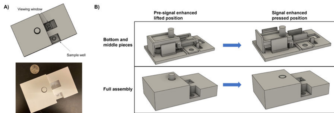
Fig. 4. (A) CAD drawing (top) and 3D printed (bottom) full casing assembly with labelled viewing window and sample well. US quarter included for size comparison. (B) CAD drawings showing the casing before and after pressing the middle piece.
