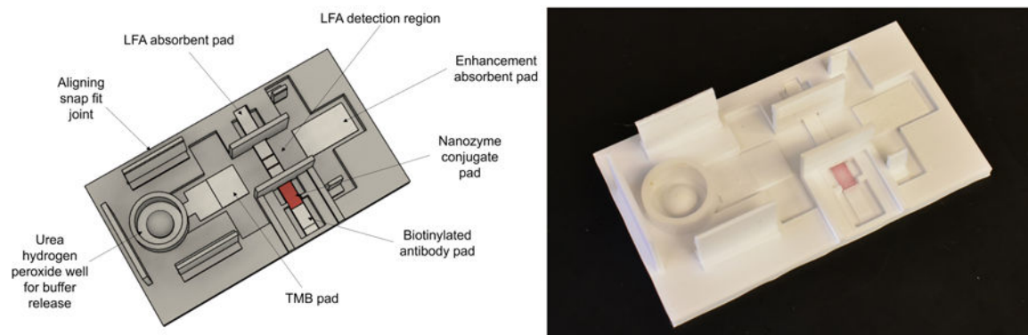
Fig. 2. (Left) Labelled CAD drawing of bottom piece of casing. (Right) Photograph of 3D printed bottom piece of casing with LFA test strip and enhancement reagent paper pads in position.
