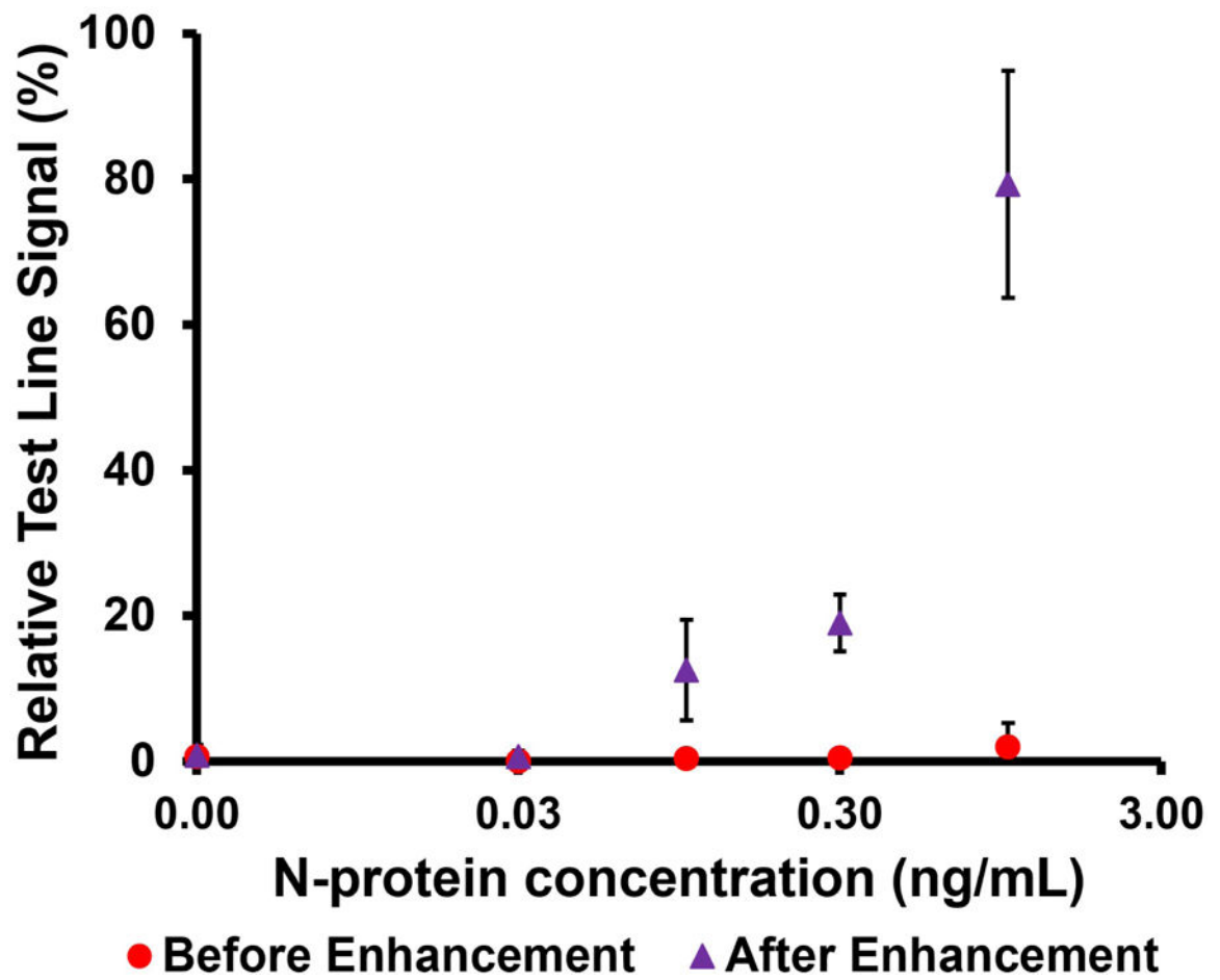
Fig. 7. Plot of relative test line signal intensity versus N-protein concentration for both the LFA (red ●) and enhancement steps (purple ▲). Data is represented as the mean \pm SD (n = 4).
