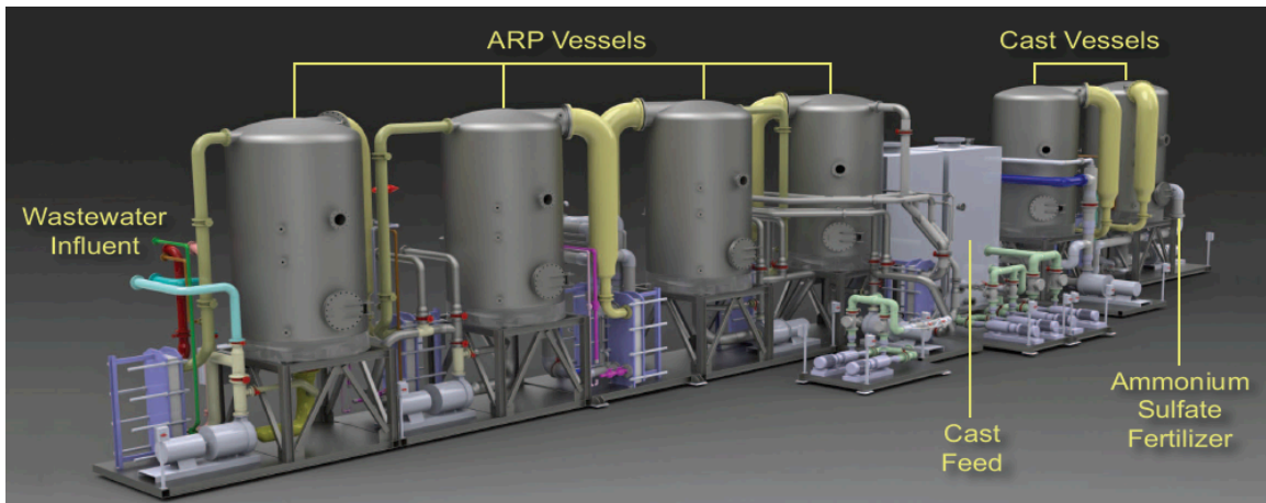
Figure 40. ThermoEnergy controlled-atmosphere separation technology applied to ammonia recovery
