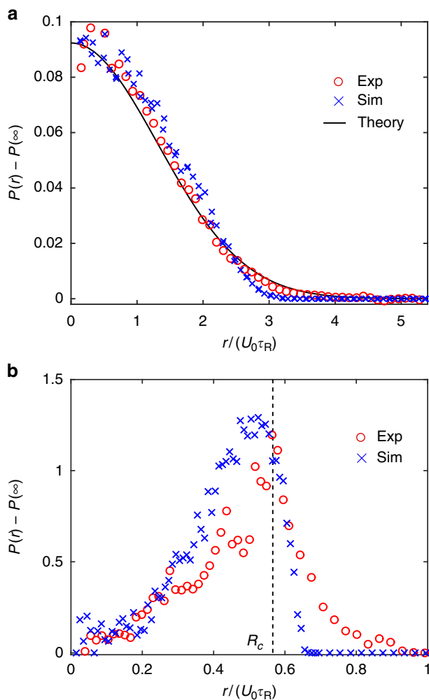
Figure 2 | Probability distribution of confined active Janus particles. (a) 2 \mu\text{m} swimmers with \alpha \equiv k\tau_R/\zeta=0.29 follow a Boltzmann distribution (solid black curve is the analytical theory, equation 1). (b) Distribution of 3 \mu\text{m} swimmers with \alpha=1.76 has a peak near R_c=\zeta U_0/k (vertical dashed black line) and decreases to zero for r>R_c . In both a,b , the red and blue symbols are data from experiment and Brownian dynamics simulations, respectively. Data are averages of measurements of over 500 snapshots for a duration of 50 s, each frame consisting \approx 100 and 20 particles for the \alpha=0.29 and \alpha=1.76 cases, respectively.
