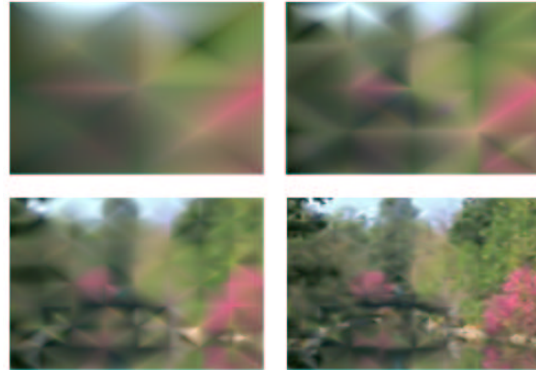
Figure 8: Hierarchical approximations of digital image data set. Original image is shown at the top. Four approximations are shown, 16, 48, 191, and 790 simplices, respectively.
