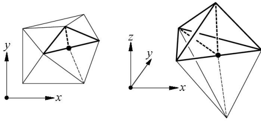
Figure 4: Bisection of simplices in bivariate and trivariate cases. Darker simplex is the one selected for bisection.
