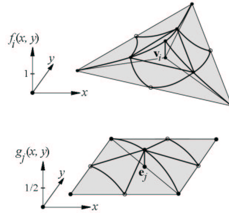
Figure 3: Basis functions associated with the platelet of vertex \mathbf{v}_i and the edge neighbors of edge \mathbf{e}_j .
