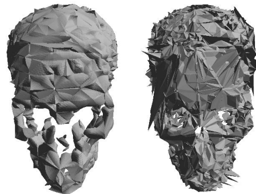
Figure 9: Comparison between quadratic approximation (left) and linear approximation (right). The quadratic approximation uses 7487 knots and 5348 simplices. The linear approximation uses 14667 knots and 78530 simplices.
