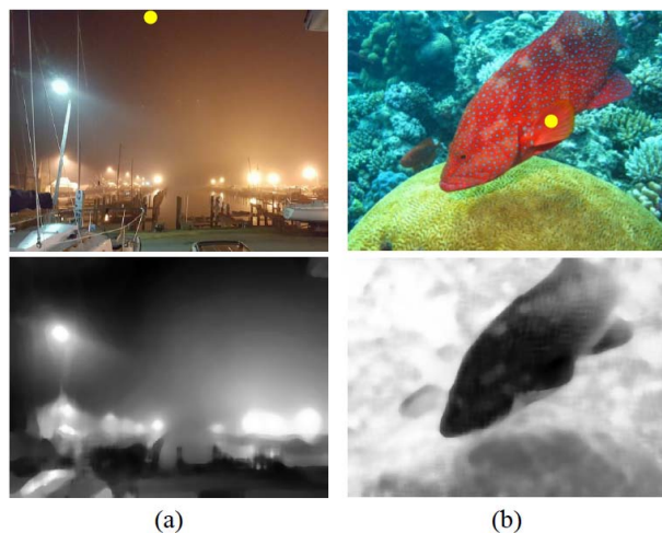
Fig. 19. Failure cases showing original images and their transmission maps. Yellow dots represent locations from which ambient light is estimated.
