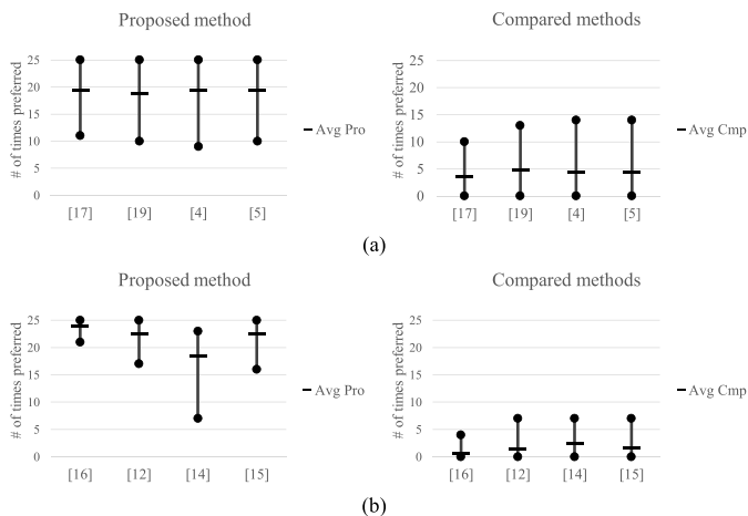
Fig. 17. Average-max-min preference charts based on all participants for the subjective experiment. (a) Terrestrial images, (b) Underwater images. (Left: The number of times our method was preferred over the comparison methods; Right: number of times compared methods were preferred. Same quality responses are ignored in this figure.)
