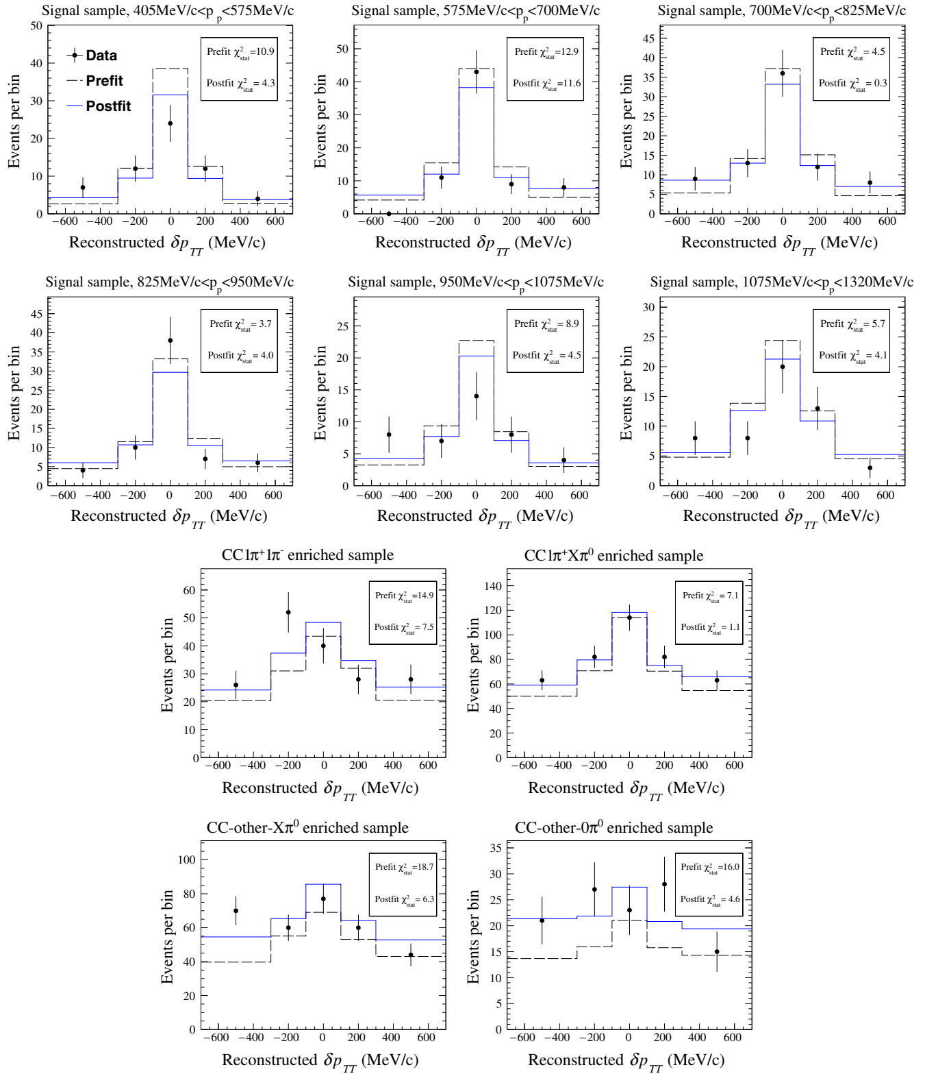
FIG. 9. Distribution of events in the signal and control samples in the \delta p_{TT} fit. \chi^2_{stat} corresponds to the statistical contribution of the fit \chi^2 [Eq. (12)] in that sample. The MC prediction before (dashed) and after (solid) the fit are also shown. The error bars show the statistical uncertainty in data.
