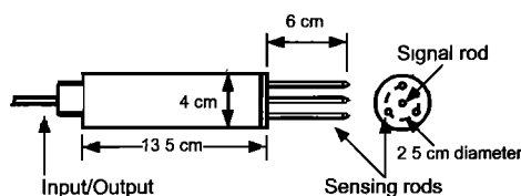
Figure 2. Soil moisture impedance probe.
