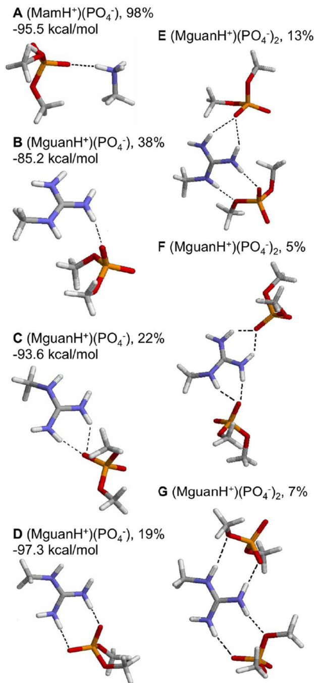
Figure 7. Representative H-bonding configurations of cluster (MamH + )(PO 4 - ) ( A ), (MguanH + )(PO 4 - ) ( B, C, D ), (MguanH + )(PO 4 - ) 2 ( E, F, G ). Hydrogen bonds are shown as dashed lines. C shows an “OCO (overcoordinated O) H-bond”, D shows a “bidentate H-bond”. E shows MguanH + forming an OCO H-bond with one phosphate group and a bidentate H-bond with the other. F shows MguanH + forming 2 OCO H-bonds with 2 phosphate groups. G shows MguanH + forming 2 bidentate H-bonds with 2 phosphate groups, called “Arg-fork”. Their percentage and the associated average interaction energy between the charged analog and
