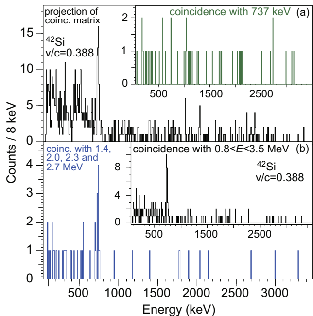
FIG. 2: (a) Projection of the \gamma\gamma coincidence matrix and coincidences with 737 keV (inset). (b) Summed coincidence spectrum obtained from gates on the photopeaks of all higher-energy \gamma -ray transitions and coincidences with 0.8 < E < 3.5 MeV (inset). Spectra are not background-subtracted.
