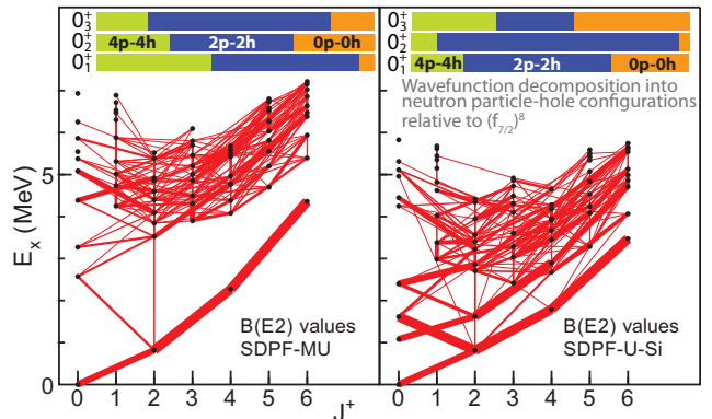
FIG. 4: Wavefunction decomposition of the first three 0^+ states and network of E2 transitions as predicted by the SDPF-MU (left) and SDPF-U-Si (right) shell-model calculations. The first ten states of each J^+ are computed together with their B(E2) strength connecting to all other calculated states (displayed as connecting lines). The line thicknesses represent the B(E2) strength of each transition.
