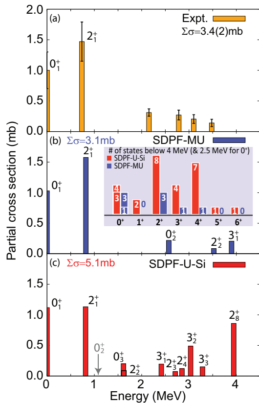
FIG. 3: Partial proton removal cross sections from ^{43}\text{P} to bound states in ^{42}\text{Si} : (a) experiment, (b) direct reaction theory with SDPF-MU shell-model spectroscopic factors, and (c) direct reaction theory with SDPF-U-Si shell-model spectroscopic factors. For the calculations, states up to 4 MeV and carrying C^2S > 0.02 spectroscopic strengths were included and R_s = 0.3 was applied. The inset to (b) shows, for each of the effective interactions, the number of states below 4 MeV (and additionally below 2.5 MeV for the 0^+ states).
