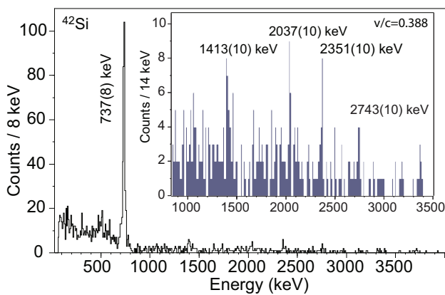
FIG. 1: Gamma-ray spectrum in coincidence with ^{42}\text{Si} reaction residues, event-by-event Doppler-reconstructed and including nearest-neighbor addback. The inset shows the high-energy region expanded.
