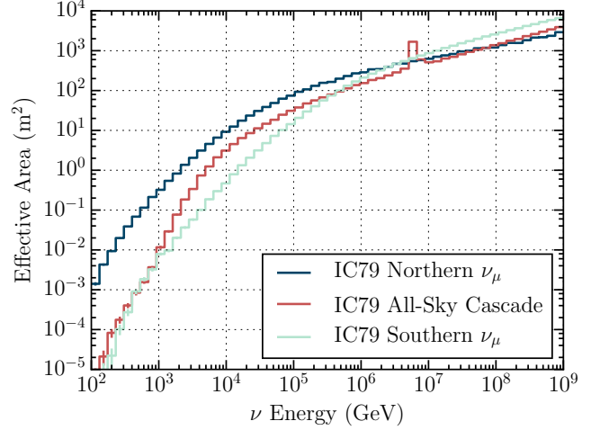
Figure 2. Effective areas, scaled to all-sky, of the Northern and Southern Hemisphere \nu_\mu track analyses compared to that of the all-sky cascade analysis for the 79-string IceCube detector configuration.
