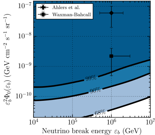
Figure 8. Excluded regions for a given CL of the generic double broken power law neutrino spectrum as a function of first break energy \epsilon_b and per-flavor quasi-diffuse flux normalization \Phi_0 derived from the presented results combined with previous Northern Hemisphere track (Aartsen et al. 2015d) and all-sky cascade (Aartsen et al. 2016a) searches. Models of neutrino production assuming GRBs are the sole source of the measured UHECR flux either by neutron escape (Ahlers et al. 2011) or proton escape (Waxman & Bahcall 1997) from the relativistic fireball are provided for reference.
