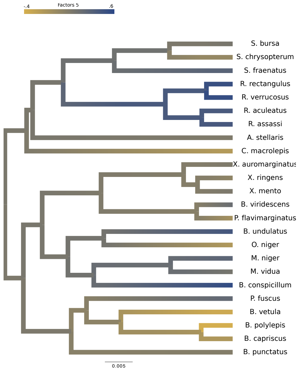
Figure 3.9: Maximum clade credibility tree for triggerfish species with yellow representing a negative factor value and navy blue representing larger factor values.
