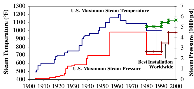
Fig. 8. Best installation PC coal-fired boiler steam temperature and pressure in the U.S. and worldwide (after 1985). Source: modified from Hirsh [24] and McMullan et al. [47].
